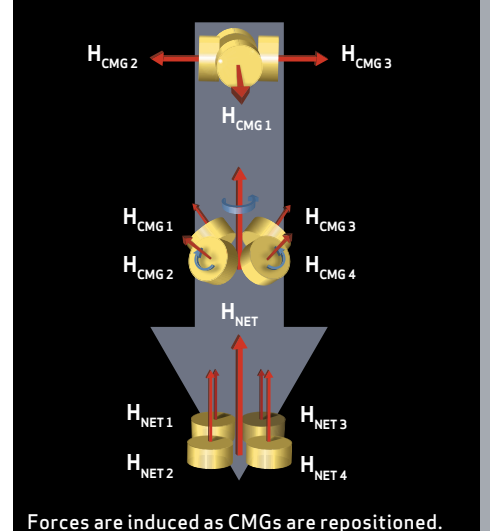
Control Moment Gyroscope gimbals used for orienting the ISS.
