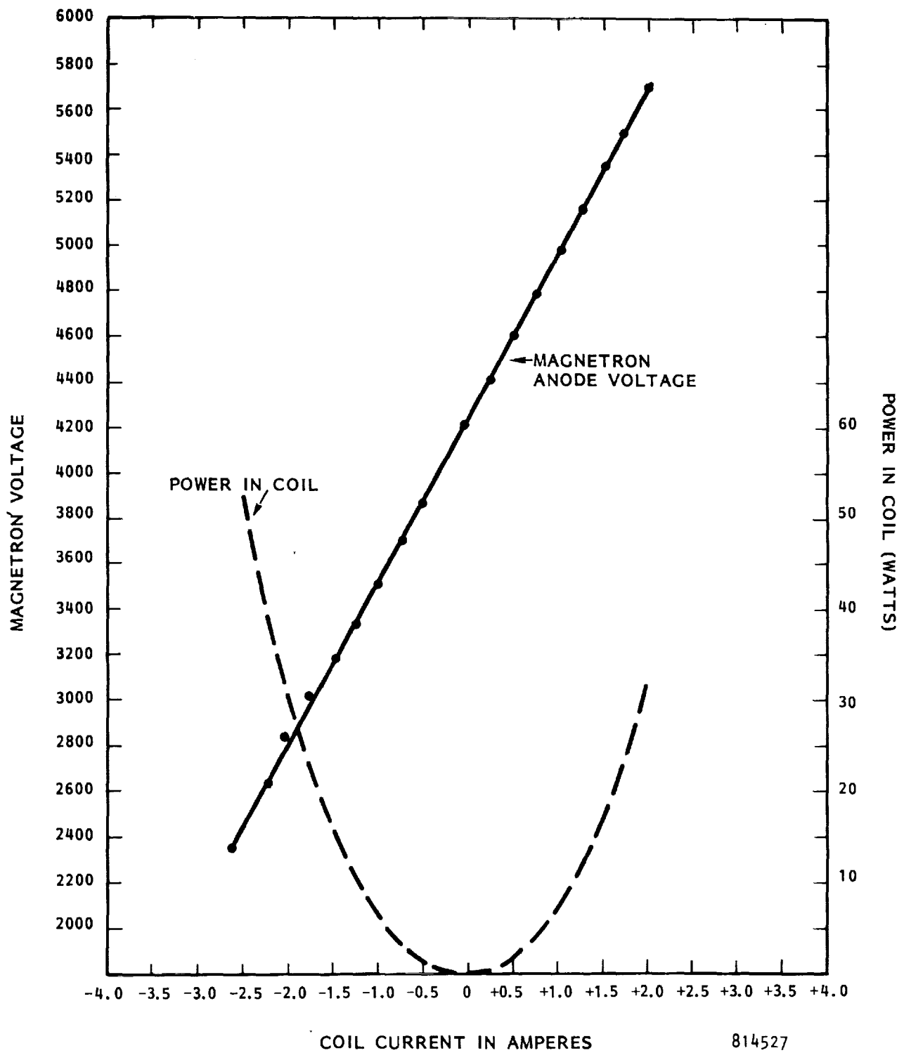
Figure 2-12. Magnetron anode voltage and power dissipated in buck-boost coil as function of current in buck-boost coil. The relationship of anode voltage to coil current is very linear as shown.
