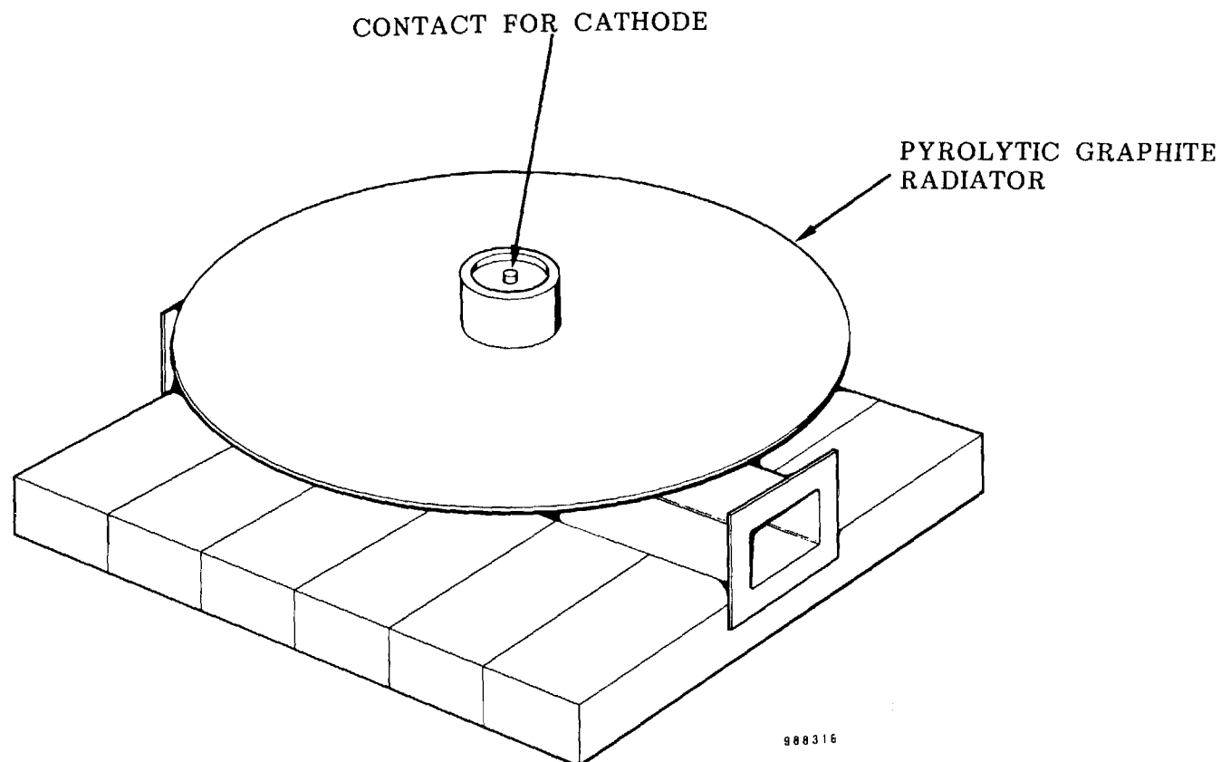
Figure 1-2. An Early Packaging Concept for Combining the Microwave Generator, its Heat Radiator, and a Section of Slotted Waveguide Radiator of Nearly the Physical Size of the Heat Radiator. In the Illustration Six Radiating Waveguides are Fed at Their Centers from a Slot in a Feed Waveguide. In the Case of the Magnetron Directional Amplifier the Feed Waveguide is Closed at Both Ends and is Fed at its Center from the Output of the Ferrite Circulator Attached to the Magnetron. Compare with Figure 4-1.
