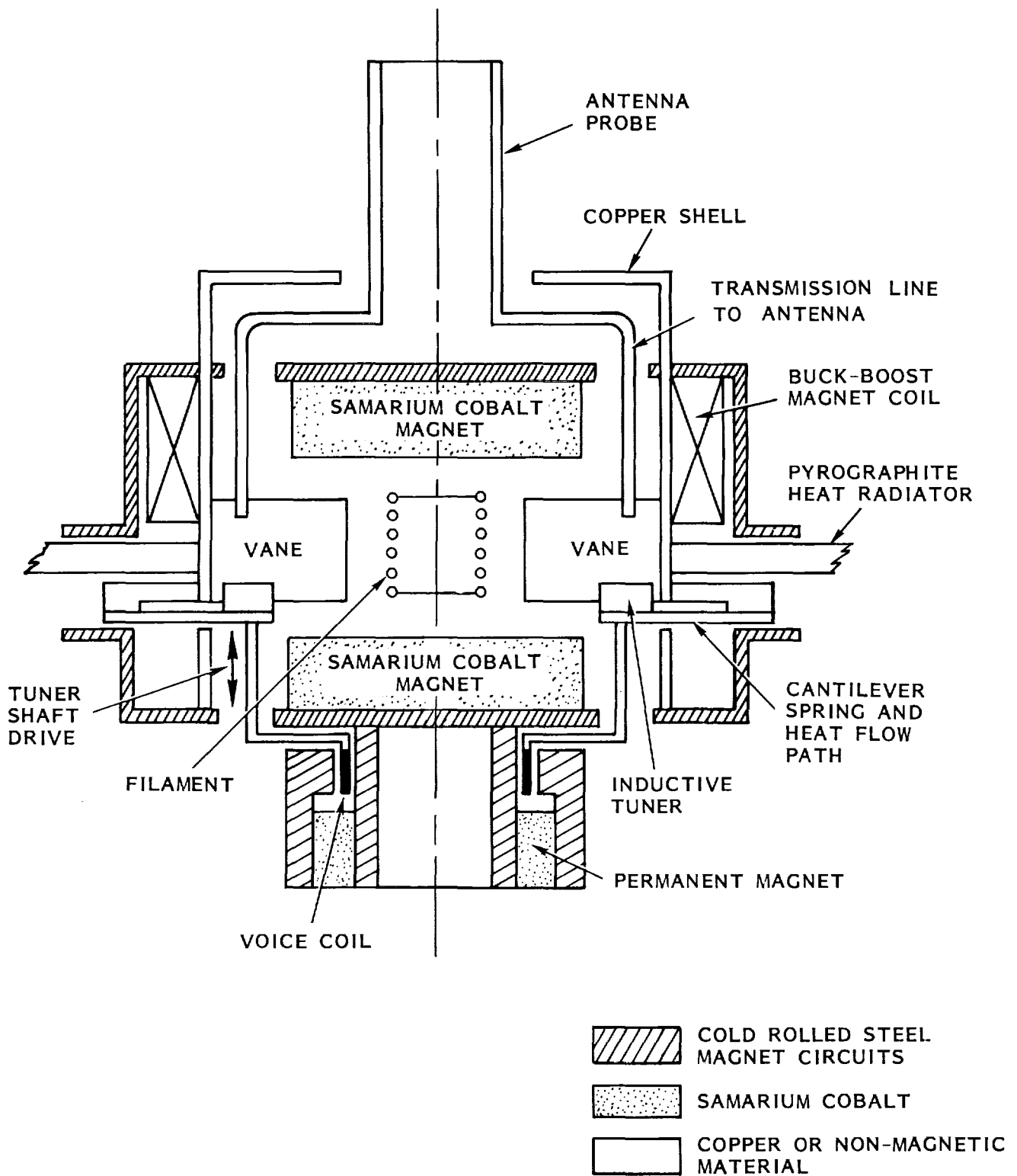
Figure 7-1. Cross Section of Magnetron Design Showing Permanent Magnets, Buck-Boost Coils for Amplitude Control, and "Voice Coil" Driven Tuner for Phase Control. Details of Support Filament are not shown.
