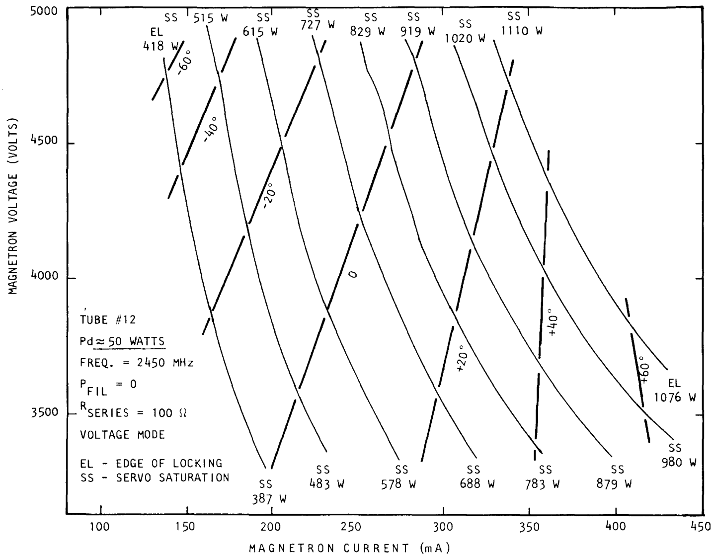
Figure 2-6. Phase and Amplitude Tracking Data with 50 Watts of Drive.
