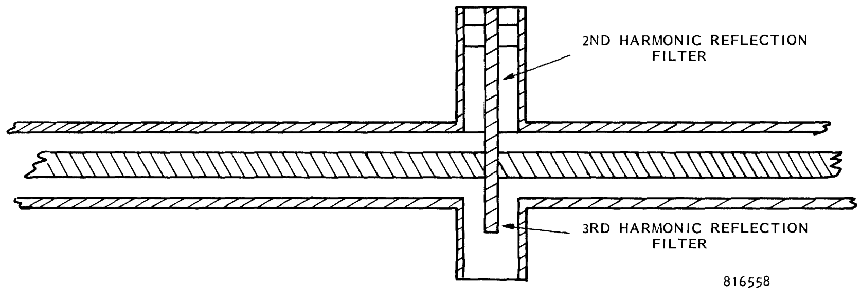
Figure 8-3. Proposed Reflection Filters to Minimize Second and Third Harmonic Power.
