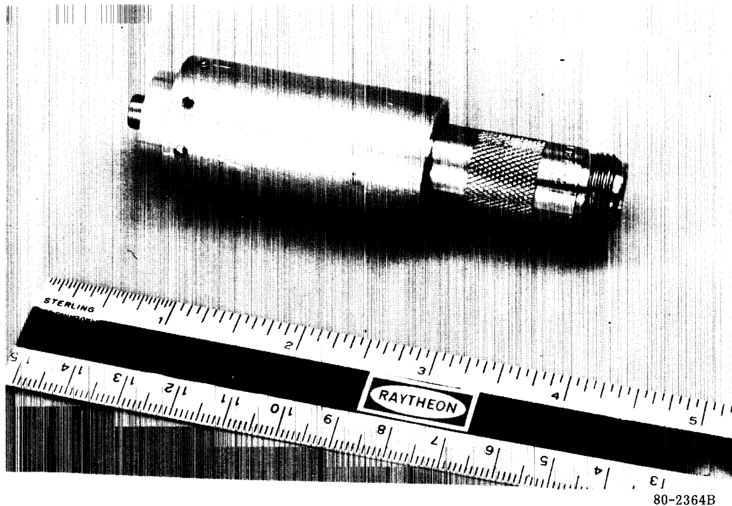
Figure 5-3a. Figure 5-3a Shows an Assembled Model of a Proposed Microwave-to-DC Source of Power for Transient Starting of Magnetrons.
