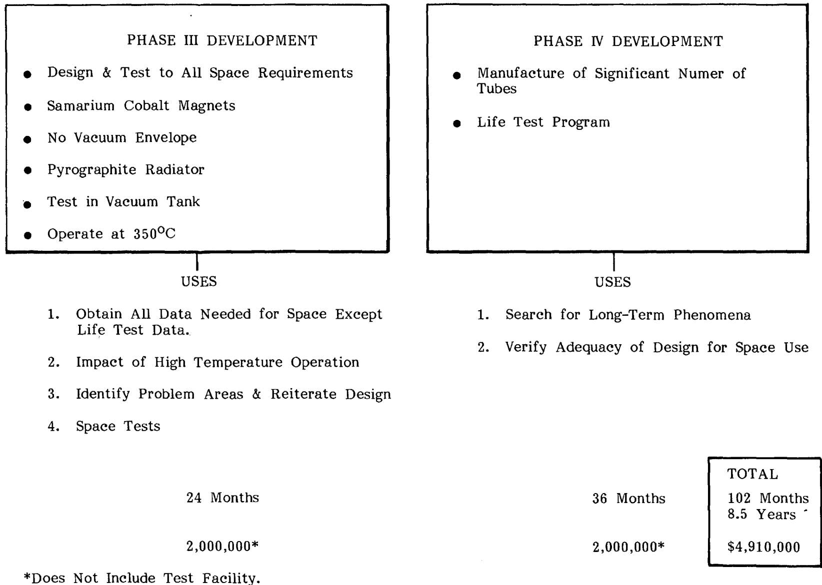
Figure 10-1. Proposed Development of SPS Magnetron Package. (Continued)
