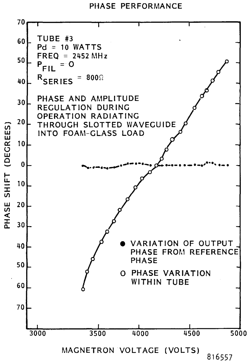
Figure 2-4. Phase Tracking of Output Phase to Reference Phase and Phase Shift through Magnetron Directional Amplifier as Function of Anode Voltage Level. Amplitude of Microwave Output is Held Constant.
