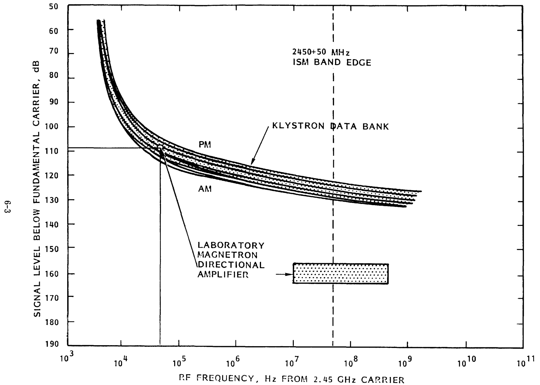
Figure 6-1. DC to RF Converter Spectral Noise Power Density in 4 kHz Bandwidth.
