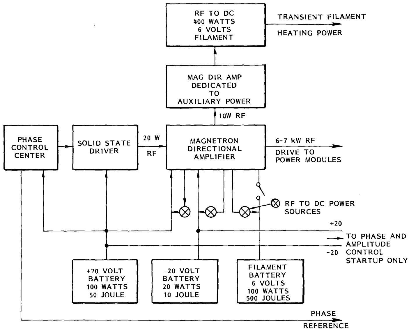
Figure 5-5. Schematic of Arrangement for Containing All Sources of Auxiliary Power within the Subarray.
