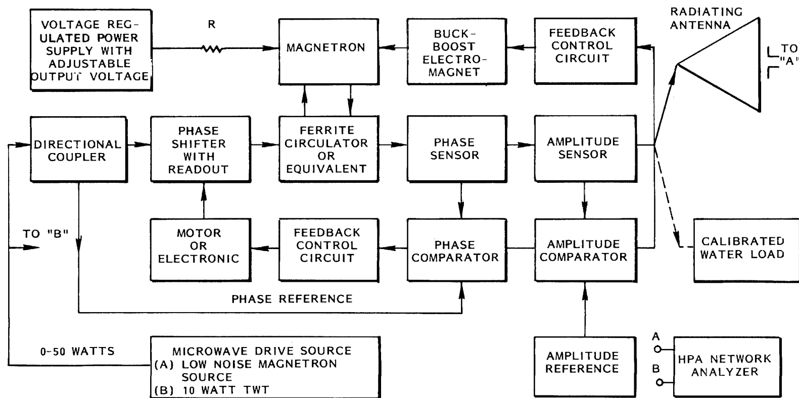
Figure 2-3. Test Arrangement for Evaluating the Magnetron Directional Amplifier with Phase and Amplitude Tracking Feature.
