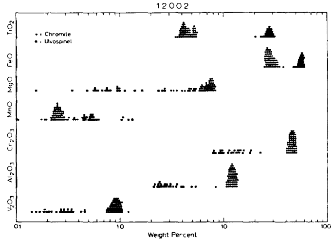
Fig. 13. Elemental distribution diagrams for chromites and ulvöspinel in typical Apollo 12 basalt (adapted from El Goresy et al., 1971).
