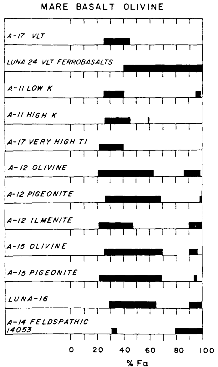
Fig. 7. Fayalite content along the join Fe_2SiO_4 - Mg_2SiO_4 for mare basalts (adapted from Pupike and Vaniman, 1978).
