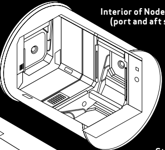
Standard Rack Bays
