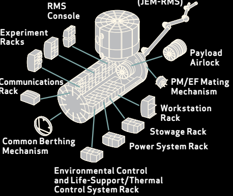
JEM Remote Manipulator System (JEM-RMS)
