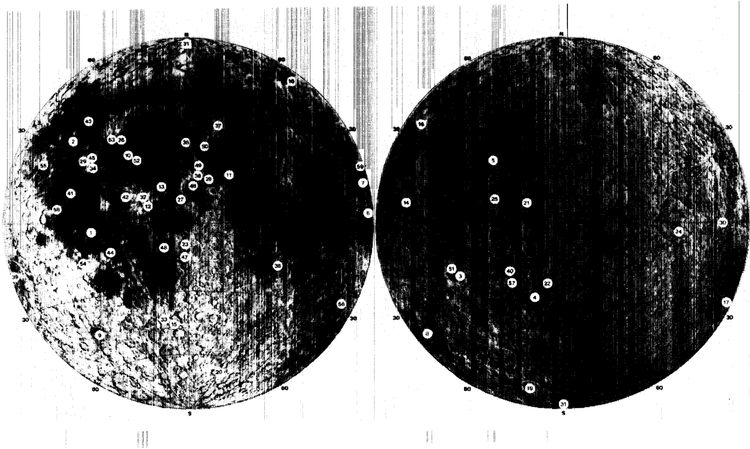
Figure V-2. Map of the Moon (equal-area projection) showing the locations of recommended sites for reconnaissance sample-return missions (numbers 1-31; see Table V-2) and for detailed study and sample return (numbers 32-59; see Table VI-2).
