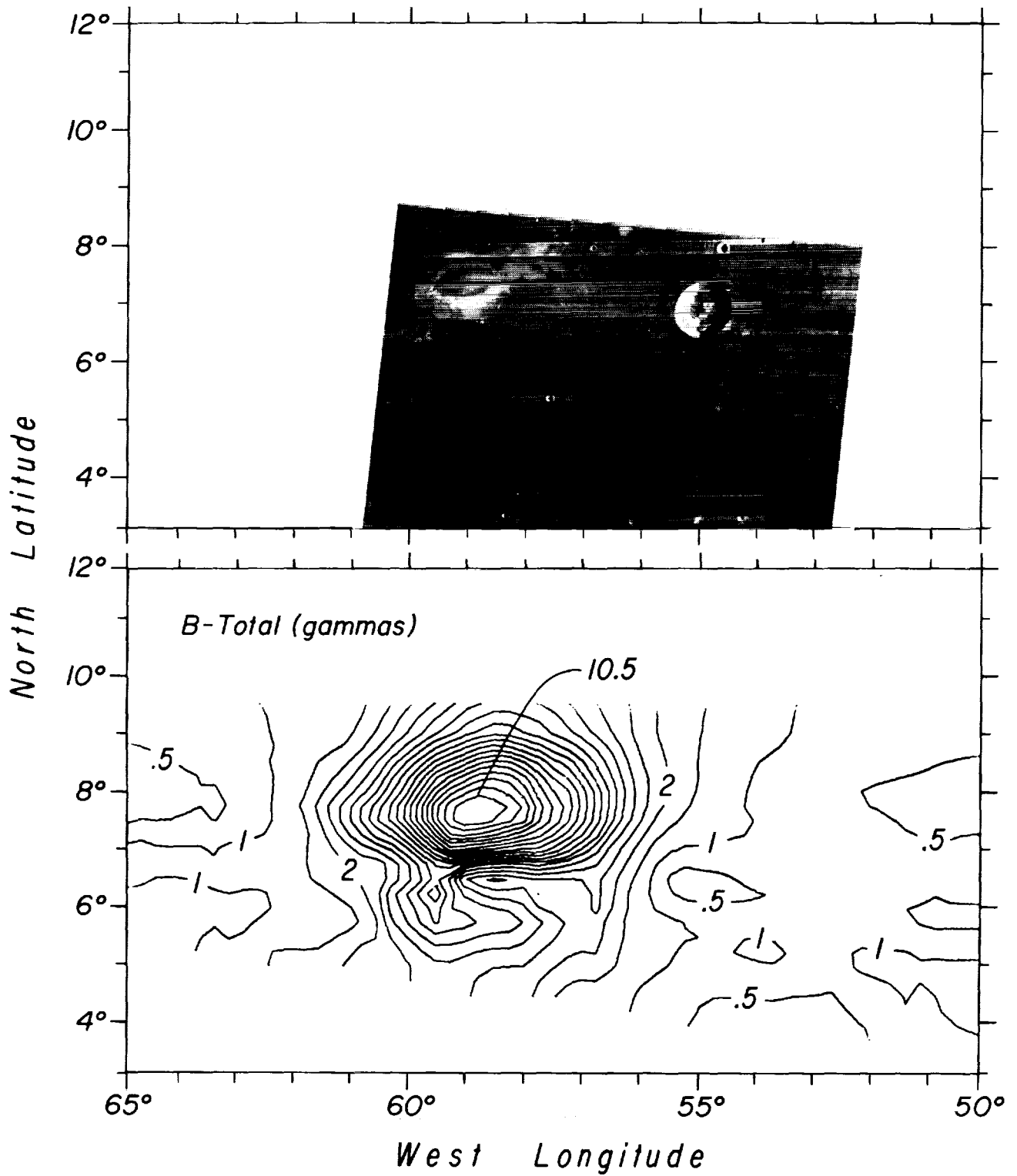
Figure VI-5. The strongest magnetic anomaly detected by the Apollo subsatellite magnetometers is correlated with Reiner Gamma, a swirl deposit of unknown origin. Return of samples could help determine how such deposits and the associated magnetic anomalies formed.
