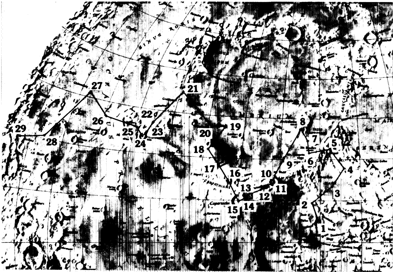
Figure VI-7. The route of a proposed traverse across the Imbrium-Procellarum region is illustrated here on a National Geographic (Lambert equal area) base map. Numbers refer to the prime field sites described in Table VI-3. Although segments are drawn as straight lines, they would actually be sinuous as the crew made numerous shorter stops along the way.
