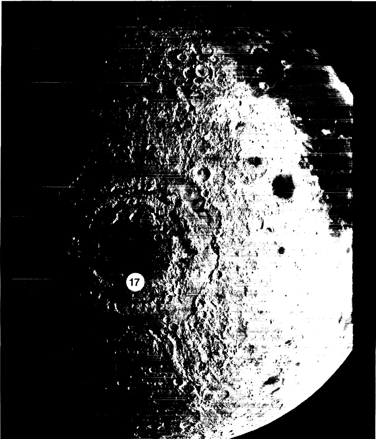
Figure V-3a. Samples from Orientale, the youngest multiringed basin on the Moon, would provide information about the age of the event that formed the basin, which marks the end of the heavy bombardment of the Moon. Samples of the impact melt sheet would also provide data about the composition of the crust in this region. Number refers to the site listed in Table V-2. Lunar Orbiter photo IV-187M.
