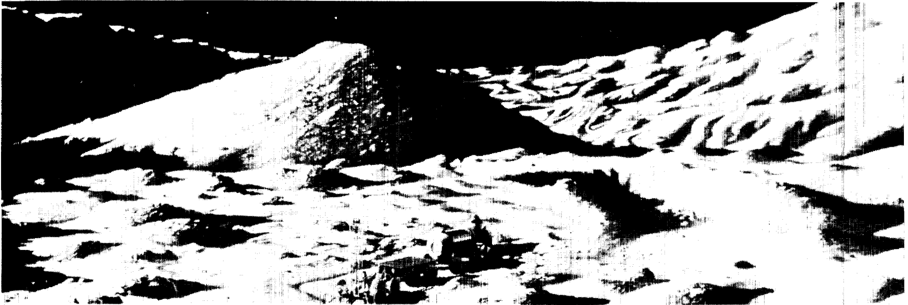
Figure VI-3. A drilling operation on the floor of Aristarchus. The core will contain valuable samples of the impact melt sheet, the composition of which represents the composition of the upper several kilometers of the lunar crust in this region. The samples will also contain information about the nature of the underlying rocks and about the cratering process. NASA painting by Patrick Rawlings.
