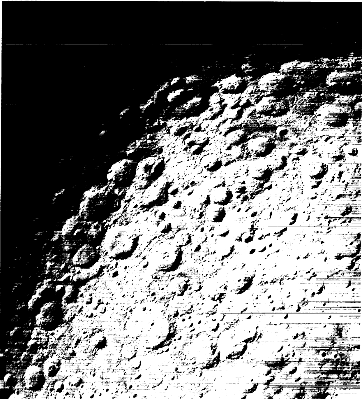
Figure II-1. Ancient cratered highlands on the far side. If the magma ocean hypothesis is correct, such areas uncontaminated with basin ejecta ought to be rich in aluminum. However, only sparse orbital geochemical data and no samples exist for the ancient highlands. Apollo metric photo AS 16-3032.
