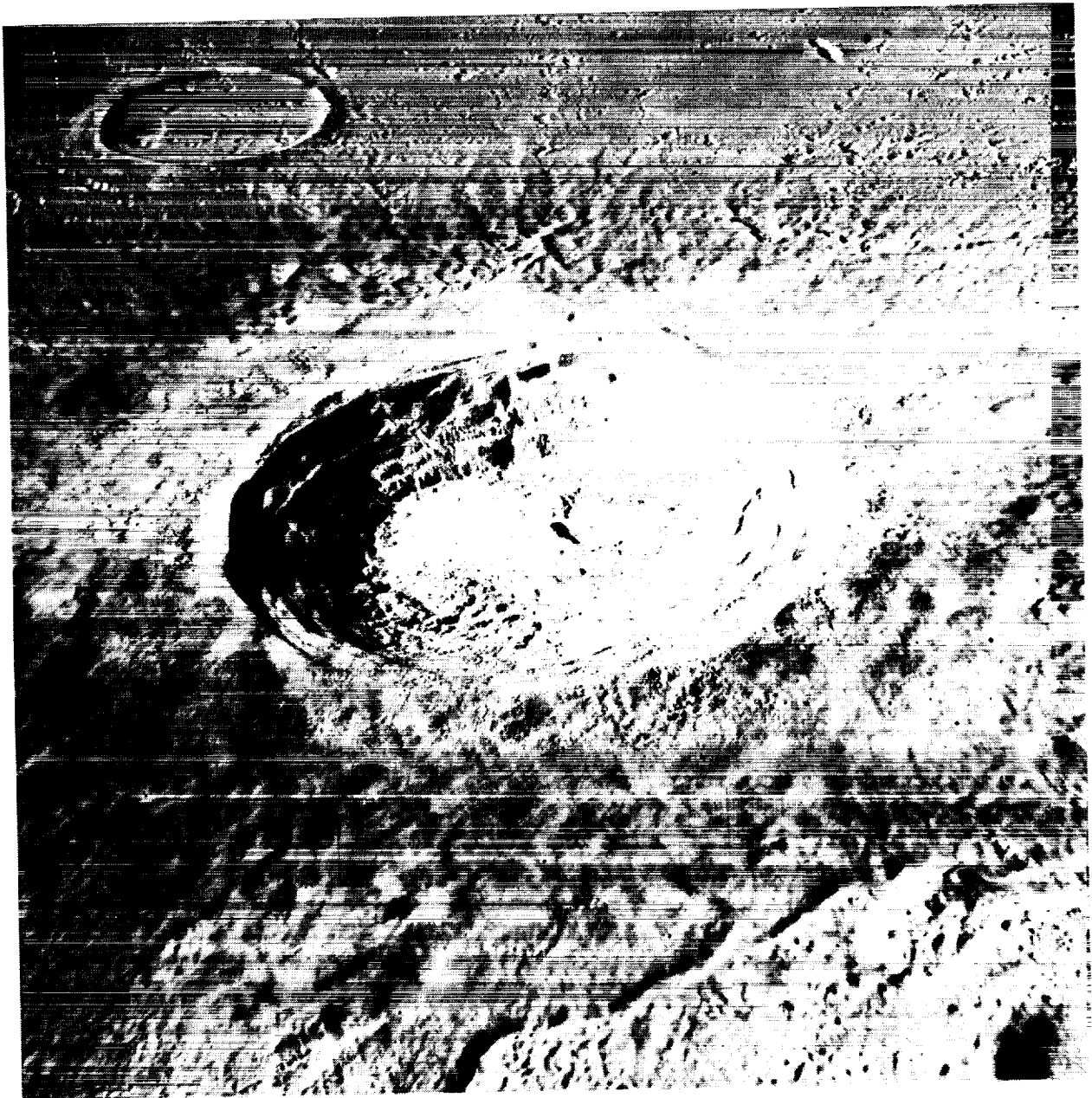
Figure VI-2. The crater Aristarchus, 42 km in diameter, is relatively young, probably less than a billion years old. Detailed study and sampling are needed of its terraced walls, central mountains, and smooth floor, which is probably composed of impact melt overlying broken, mixed, and shock rocks. Apollo photograph AS15-2609M.
