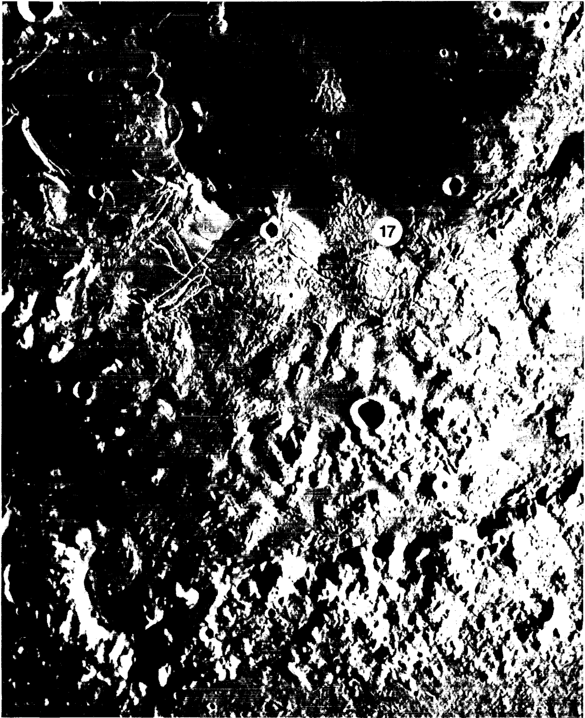
Figure V-3b. High resolution photograph of suggested landing site on the Maunder Formation inside the Orientale basin. This site would allow collection of impact melt (light-colored material next to the number) and probably some mare basalt (dark material nearby, to the north) thrown to the landing site by impacts on the mare.
