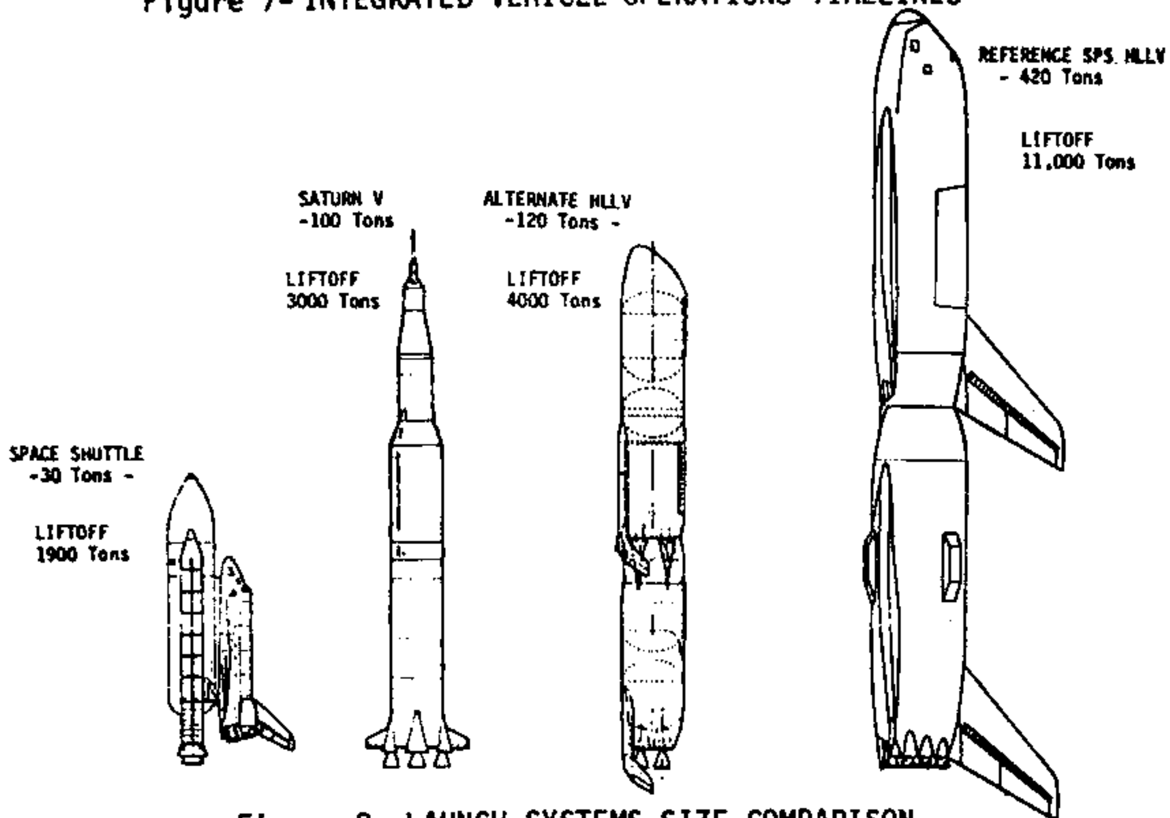
Figure 8- LAUNCH SYSTEMS SIZE COMPARISON
