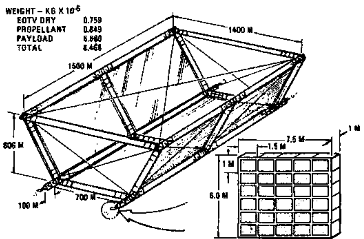
Figure Electric Orbital Transfer Vehicle
