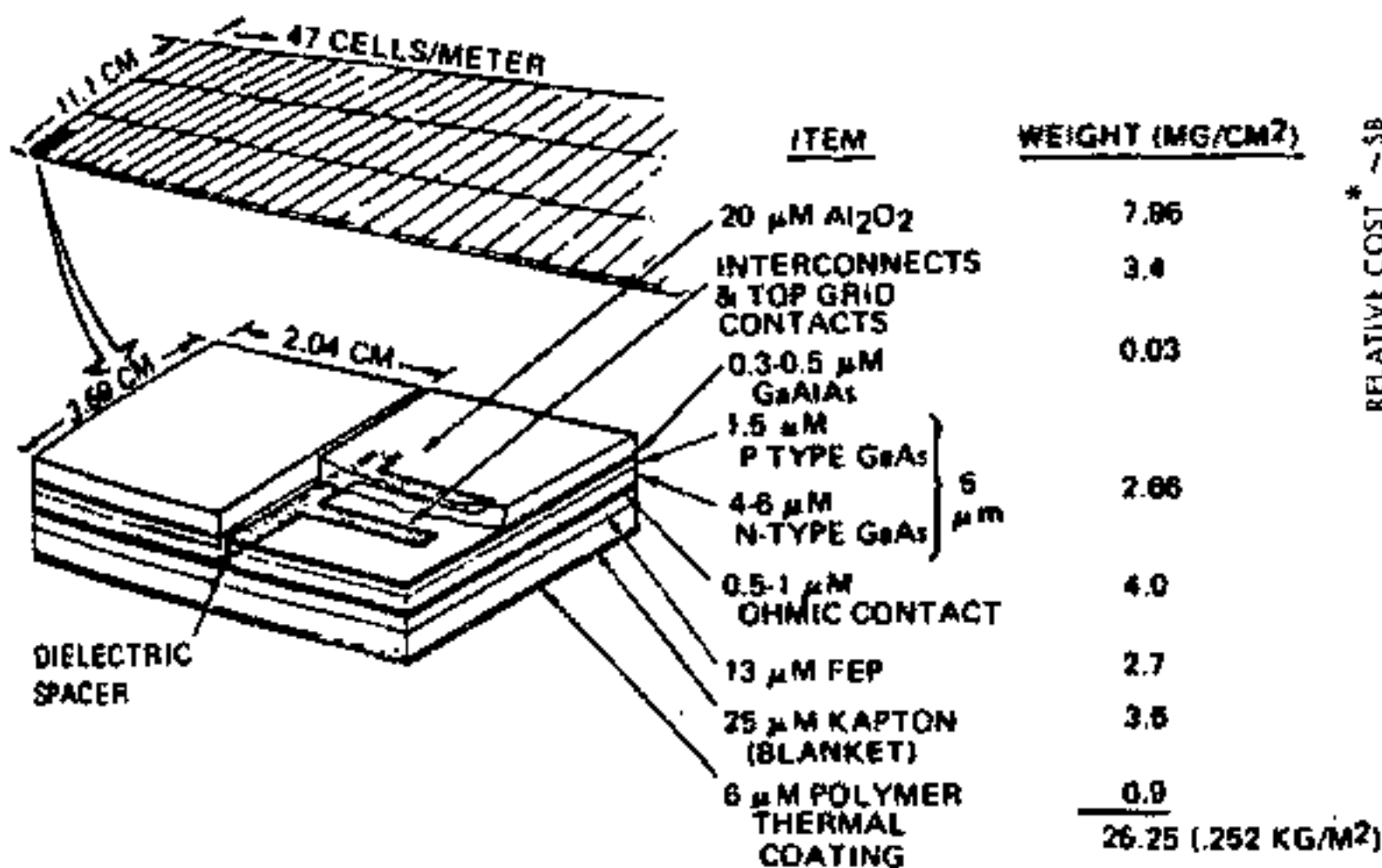
Figure 2. GaAs on Sapphire Solar Cell Blanket Cross-Section
