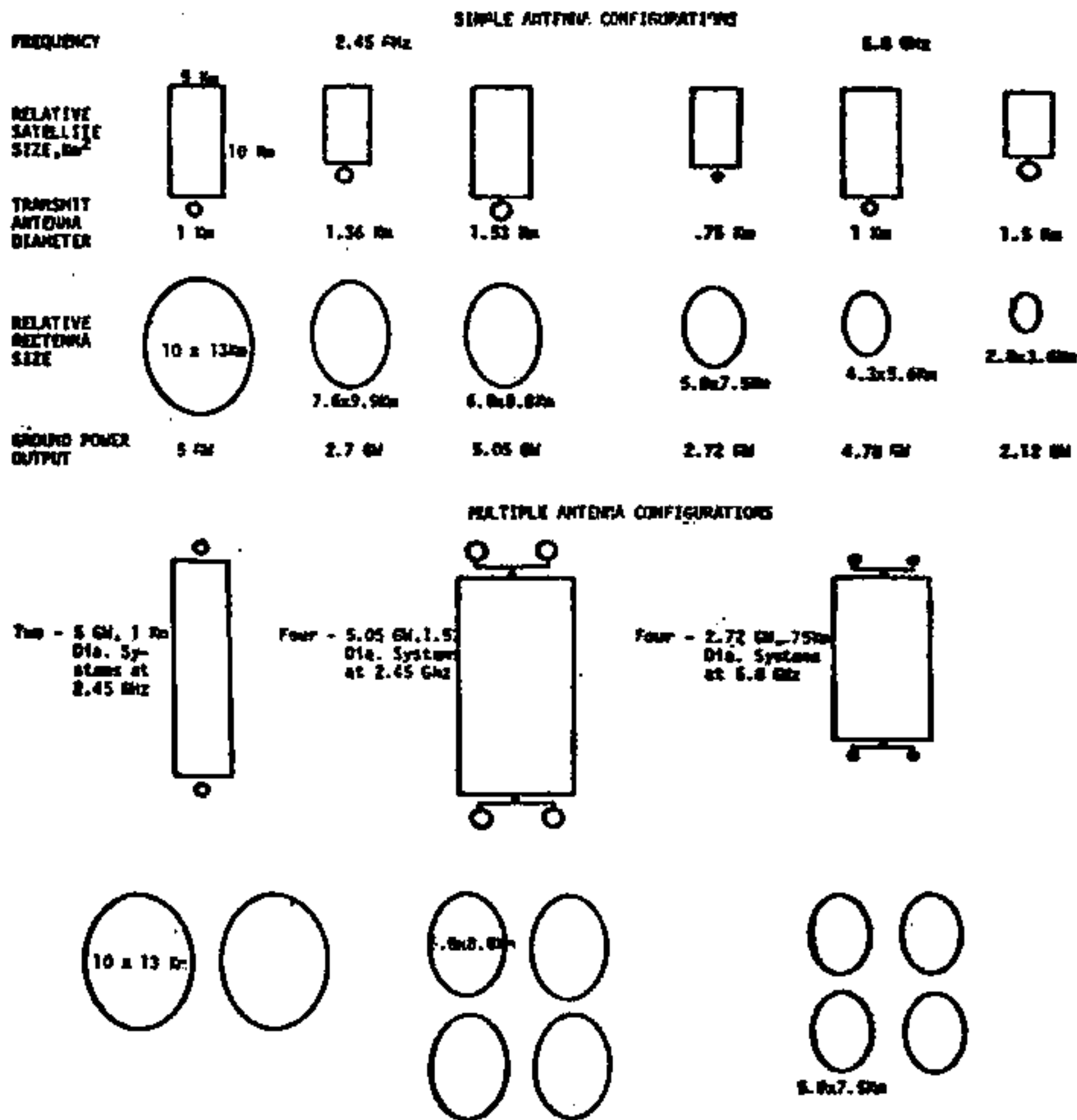
Figure 4. Relative Antenna/Rectenna Sizes Configurations
