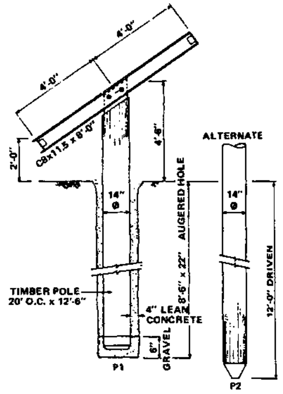
POLE FOUNDATIONS P1 AND P2 8' x 20' ARRAYS
