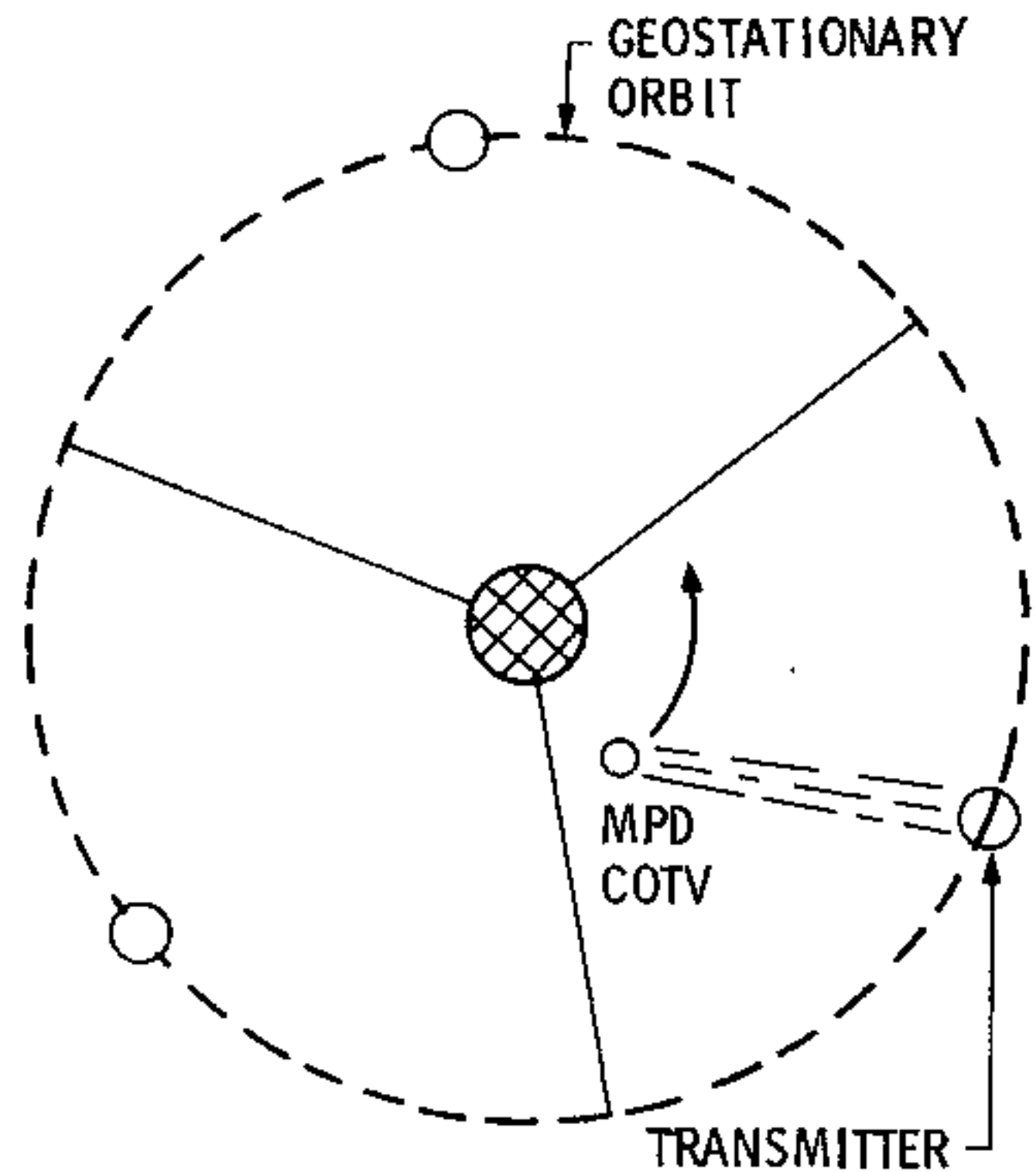
Fig. 3. Proposed microwave powered MPD-COTV concept.
