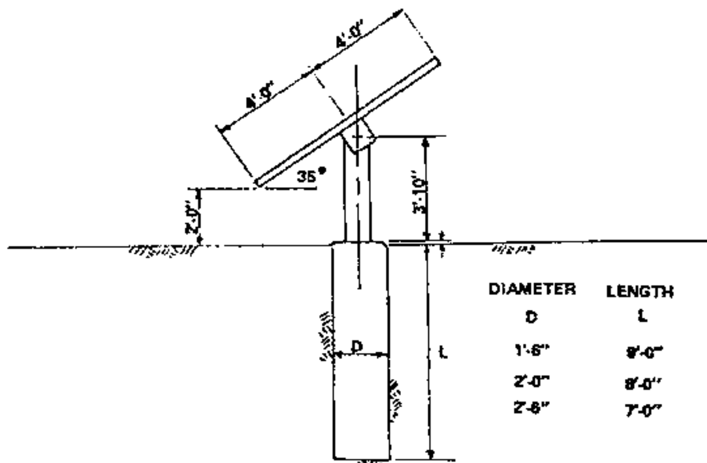
SUPPORT STRUCTURE FOR PHOTOVOLTAIC POWER PLANT
