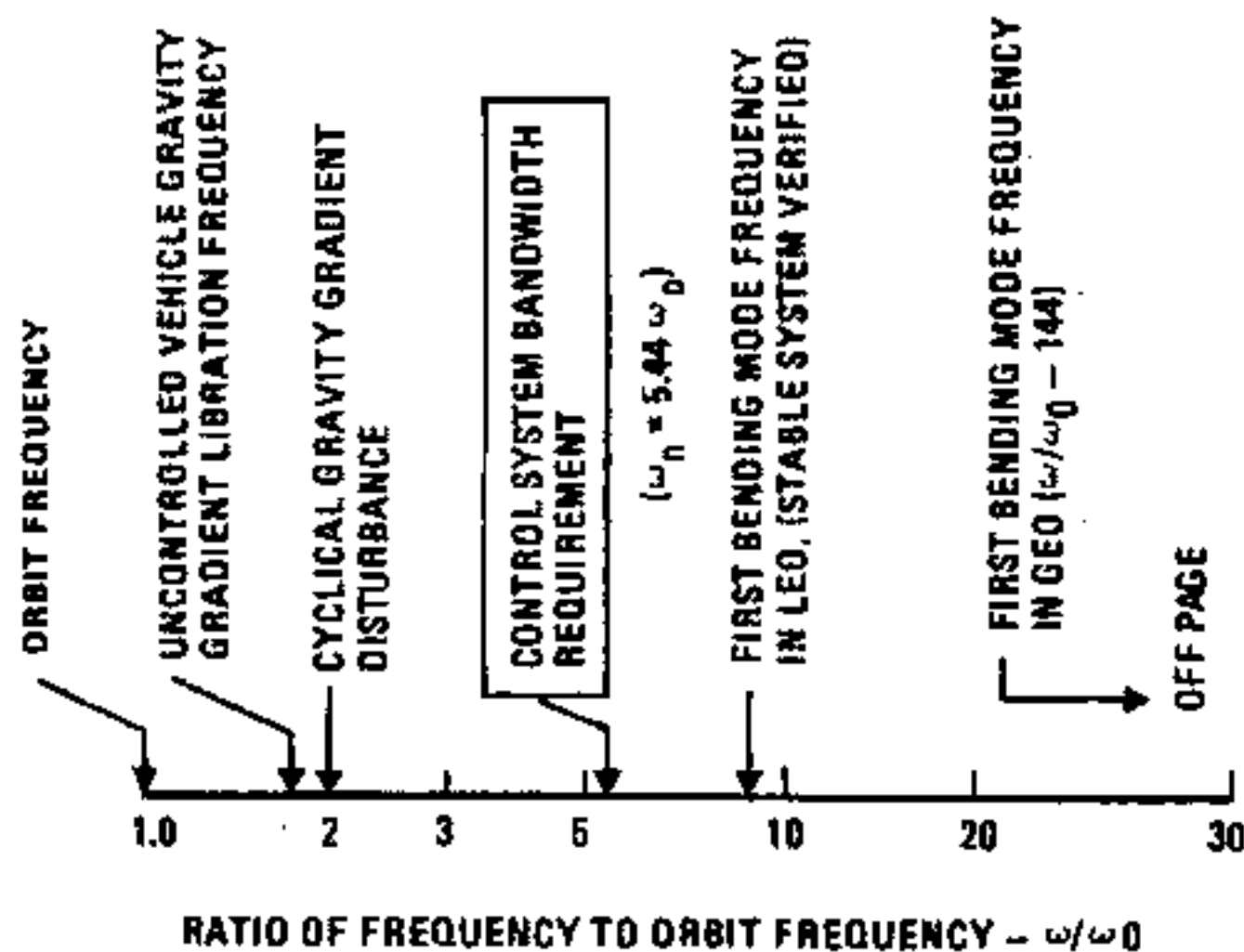
Figure 6. Frequency Distribution
