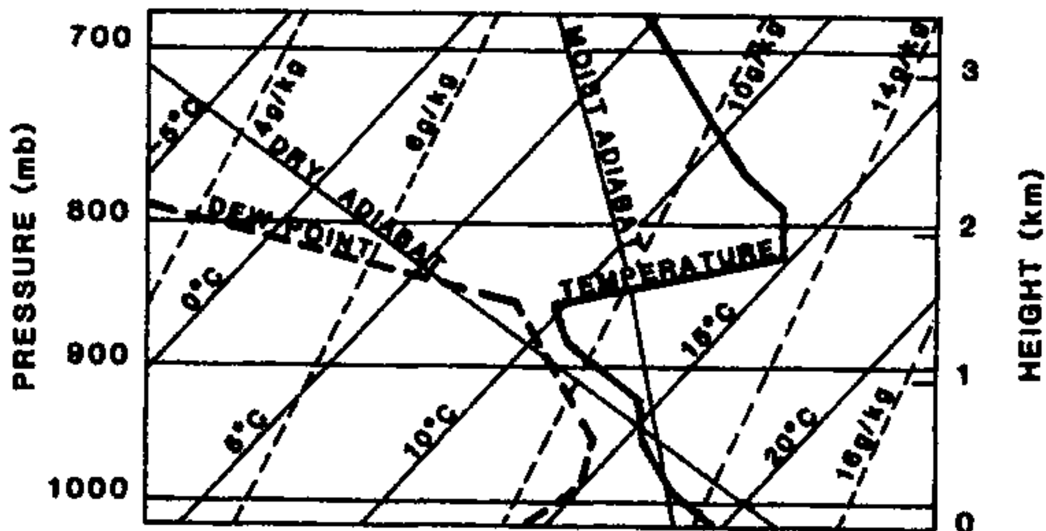
Fig. 1. Basic Sounding for 1936 EST 13 December 1978, CAPE CANAVERAL, Florida
