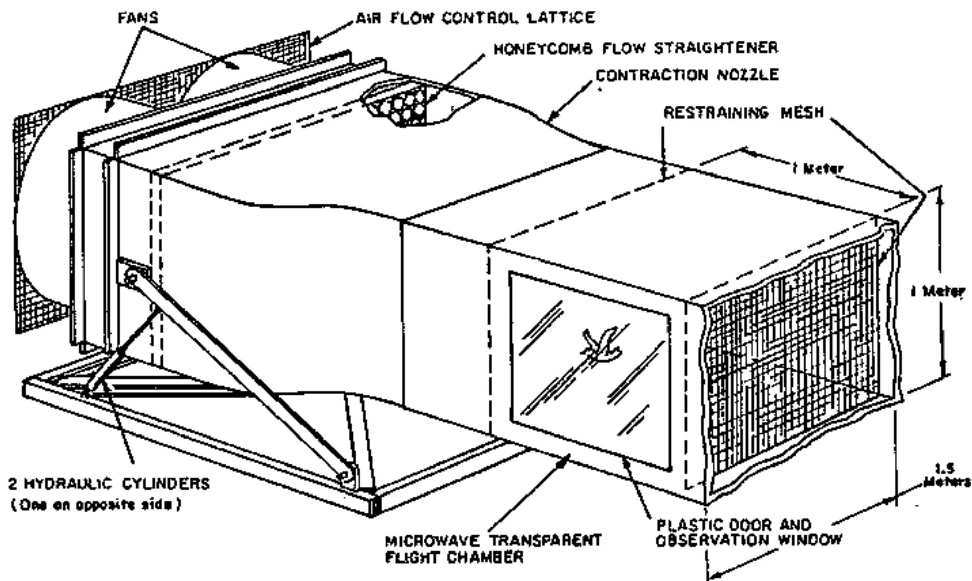
FIGURE 6. WIND TUNNEL AND FLIGHT CHAMBER
