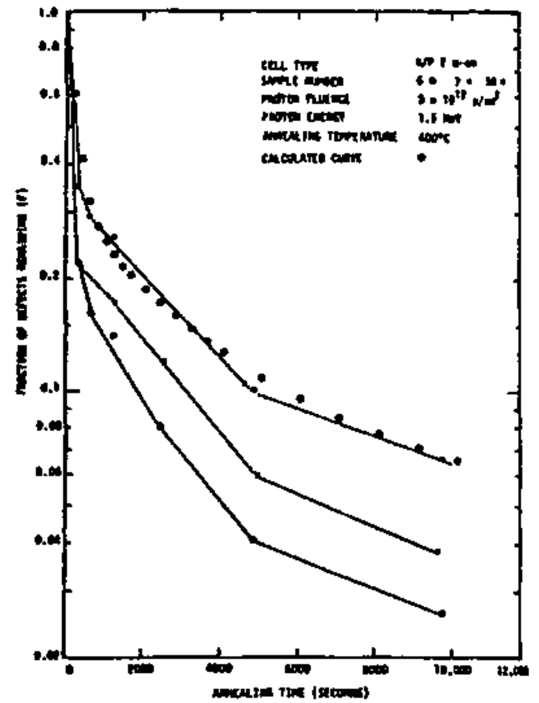
Figure 2. Isothermal Annealing of 3 \times 10^{12} p/cm 2 Proton Damage at 400°C
