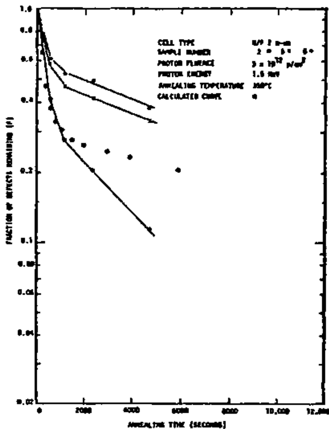
Figure 3. Isothermal Annealing of 3 \times 10^{12} p/cm 2 Proton Damage at 350°C
