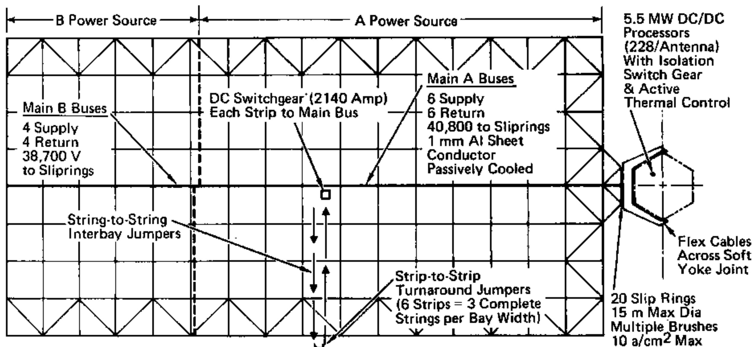
Figure 3. Multiple Bus SPS Power Distribution (Si Cells)
