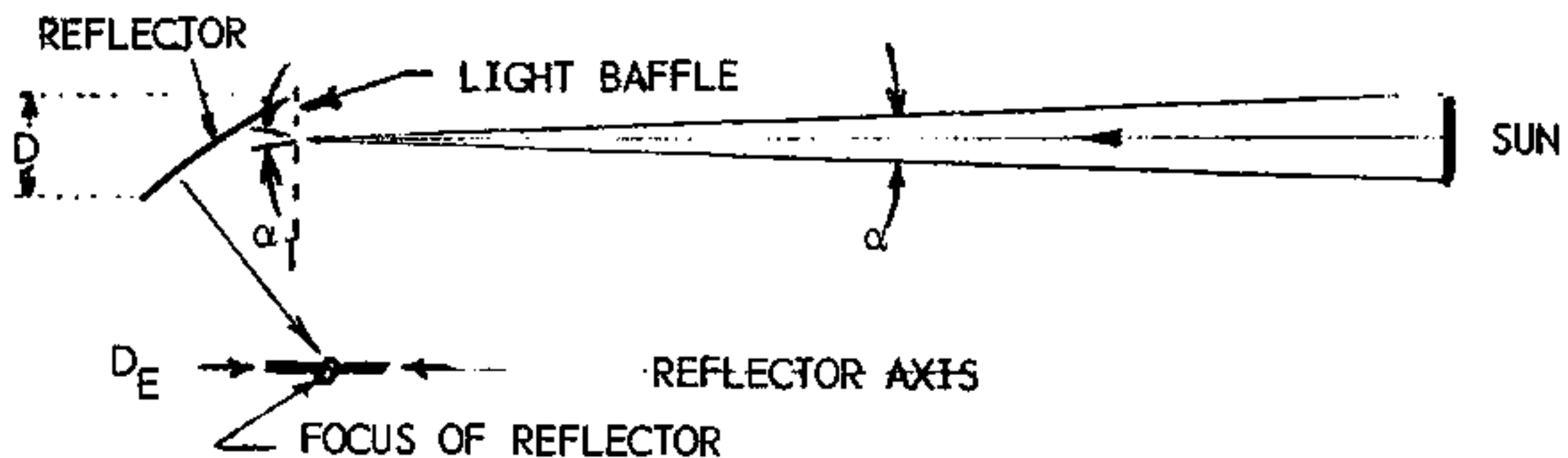
FIG. 2. SINGLE REFLECTOR WITH BAFFLE
