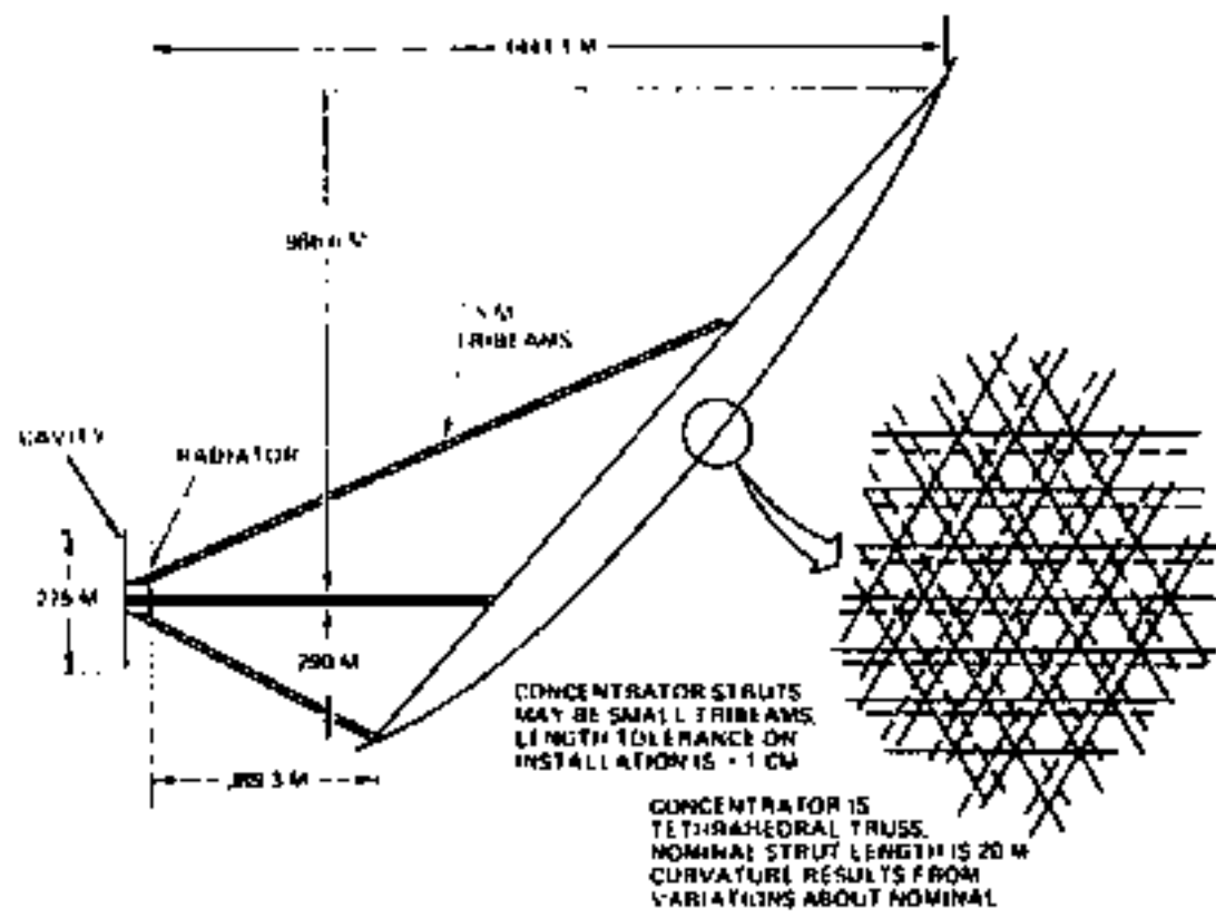
Figure 5. Indirectly Optically Pumped Laser SPS General Arrangement
