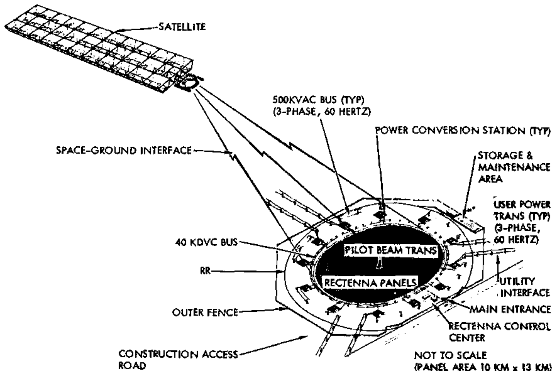
Figure 1 Satellite Power System
