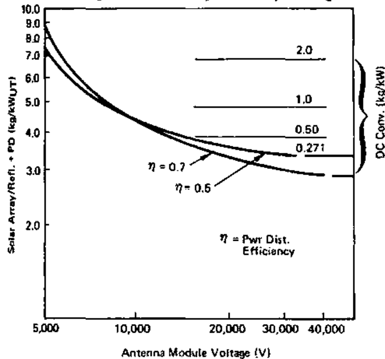
Figure 9. Antenna Module Voltage Crossover (Without dc Converters)
