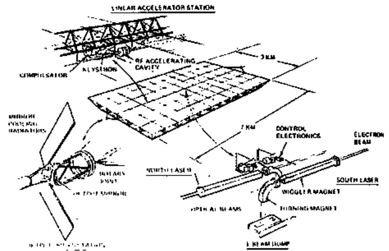
Figure 6. 1-GW Single-Pass Free Electron Laser SPS
