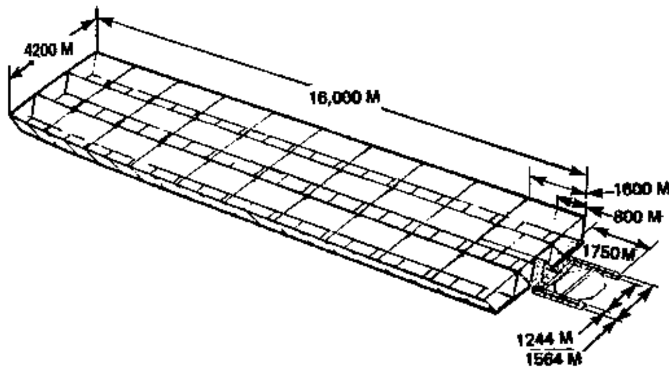
Figure 1. SPS Reference Configuration (GaAs Cells, CR=2)
