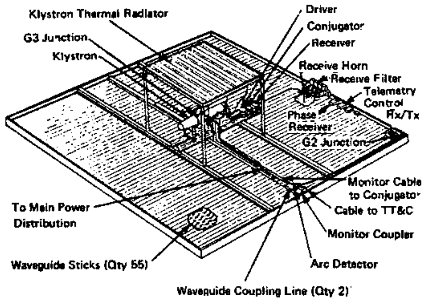
Figure 5. Mechanical Layout of typical Klystron Module
