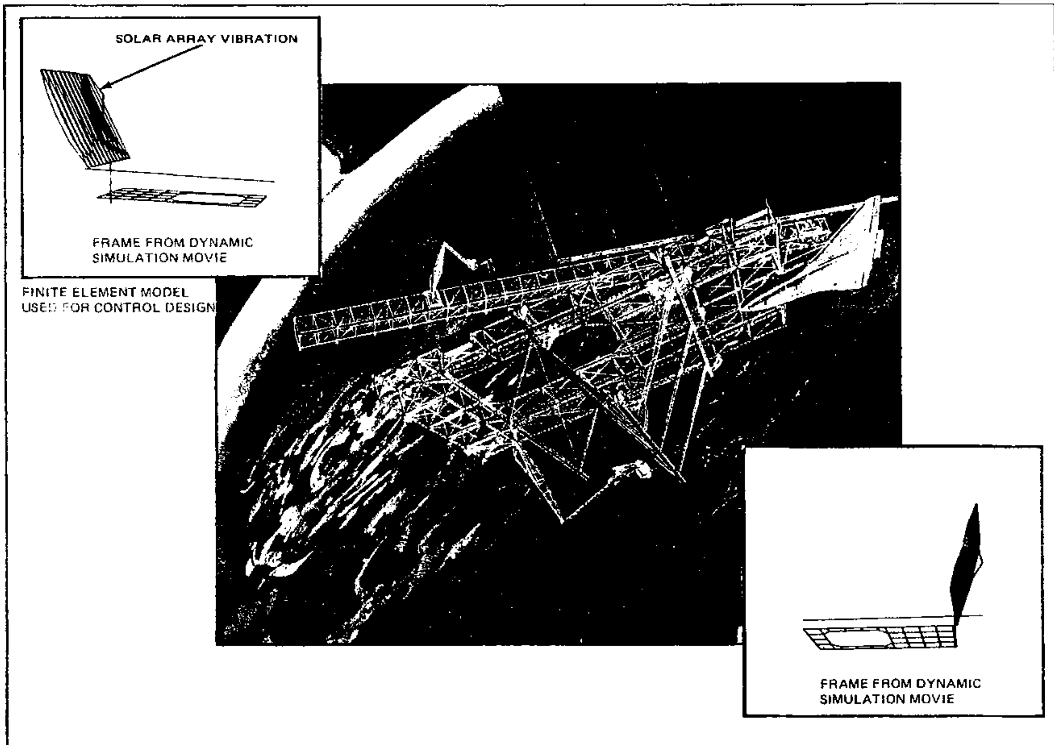
Fig. 2 Orbital Construction Demonstration Article
