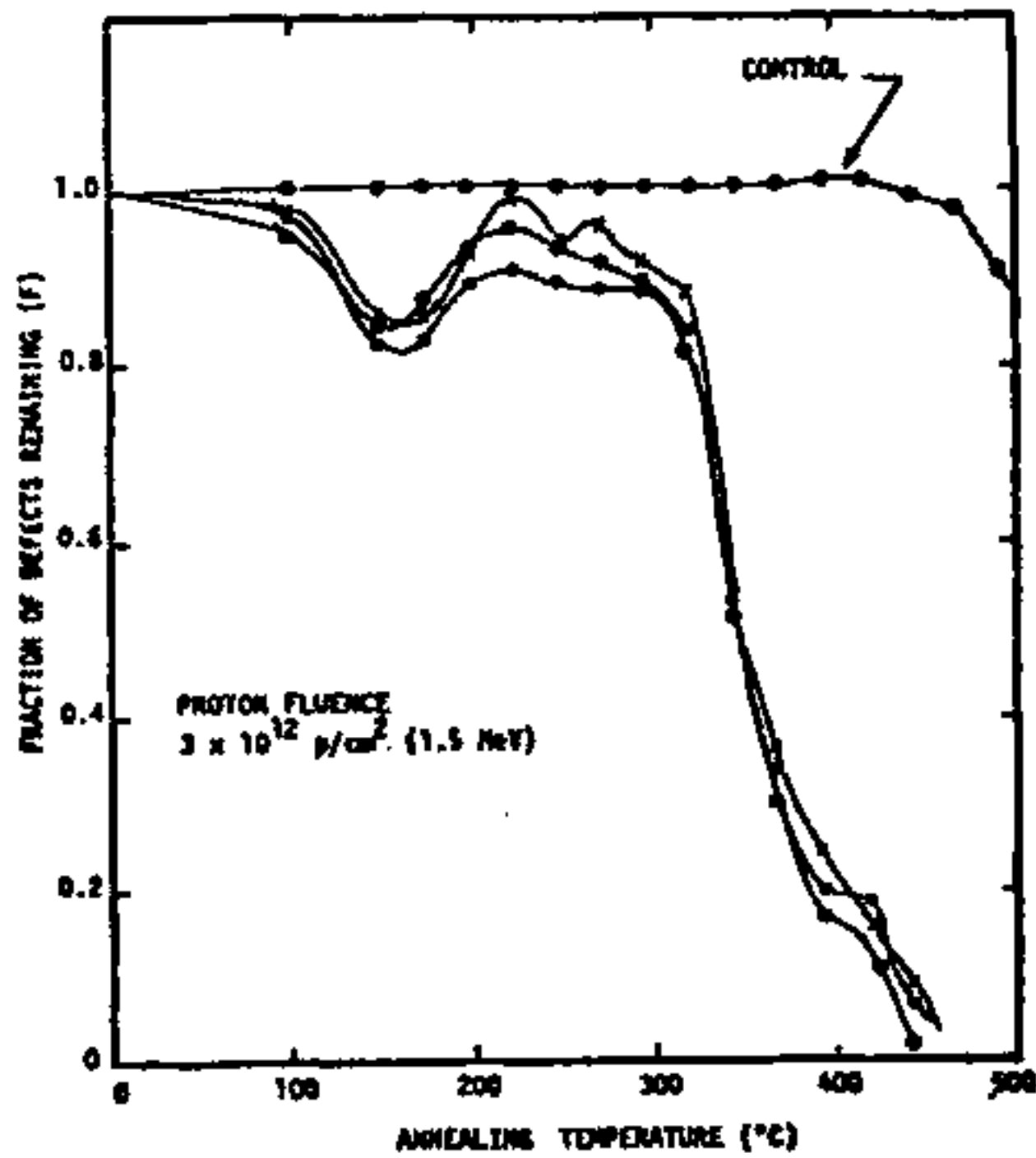
Figure 1. Isochronal Annealing of Proton Damage
