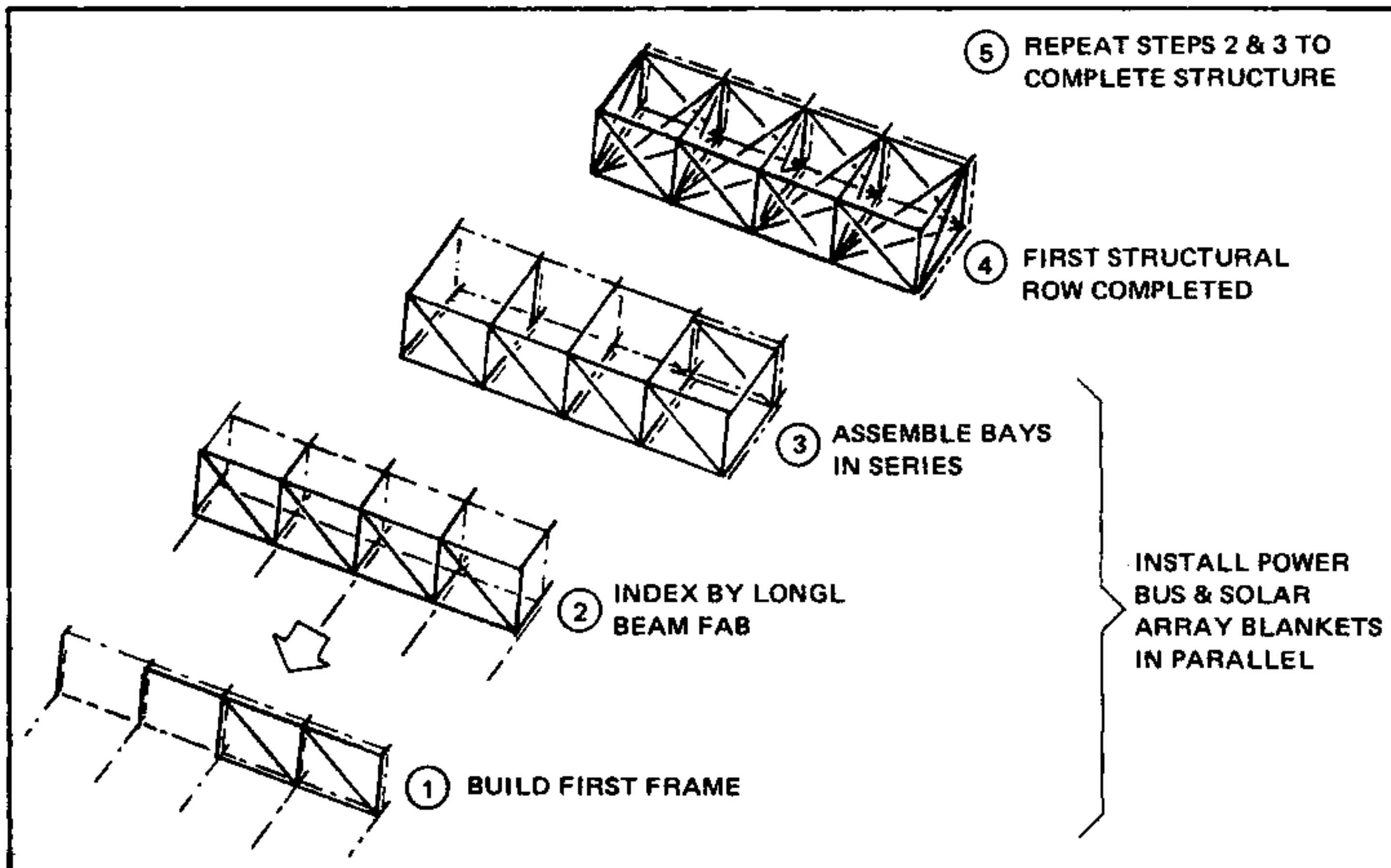
Fig. 3 End Builder Structural Assembly Sequence
