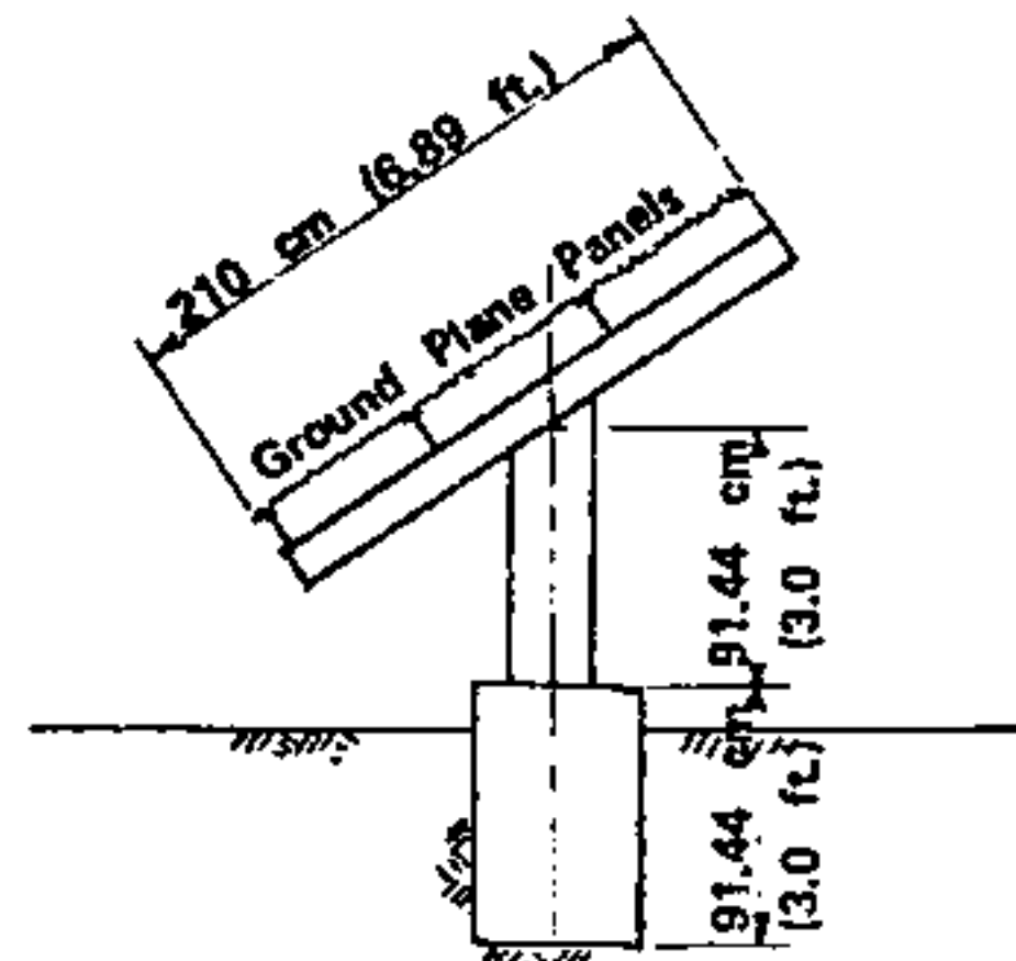
SUPPORT STRUCTURE FOR SPS RECTENNA
