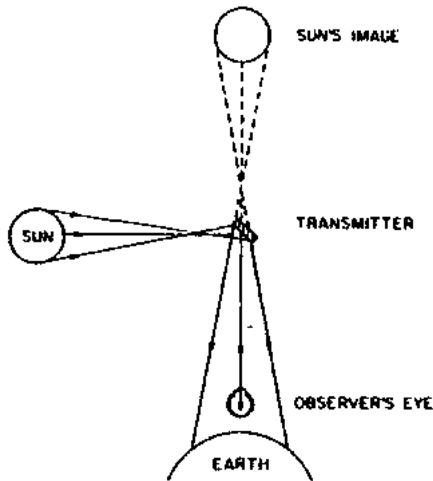
RAY DIAGRAM FOR CALCULATION OF SPS BRIGHTNESS
