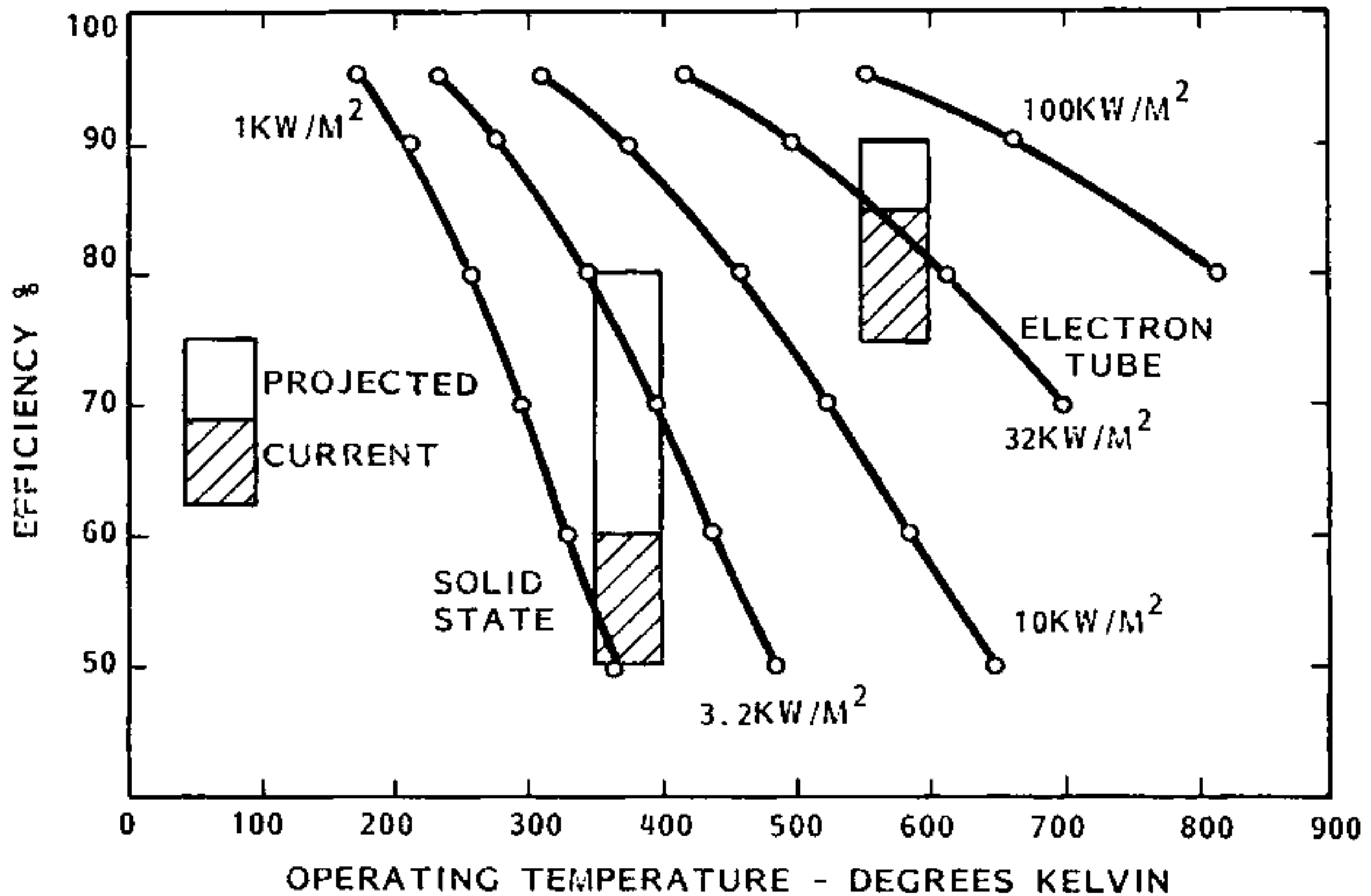
Figure 2. Contours of Microwave Power Outputs as Function of Efficiency and Operating Temperature of Microwave Generators. 813693
