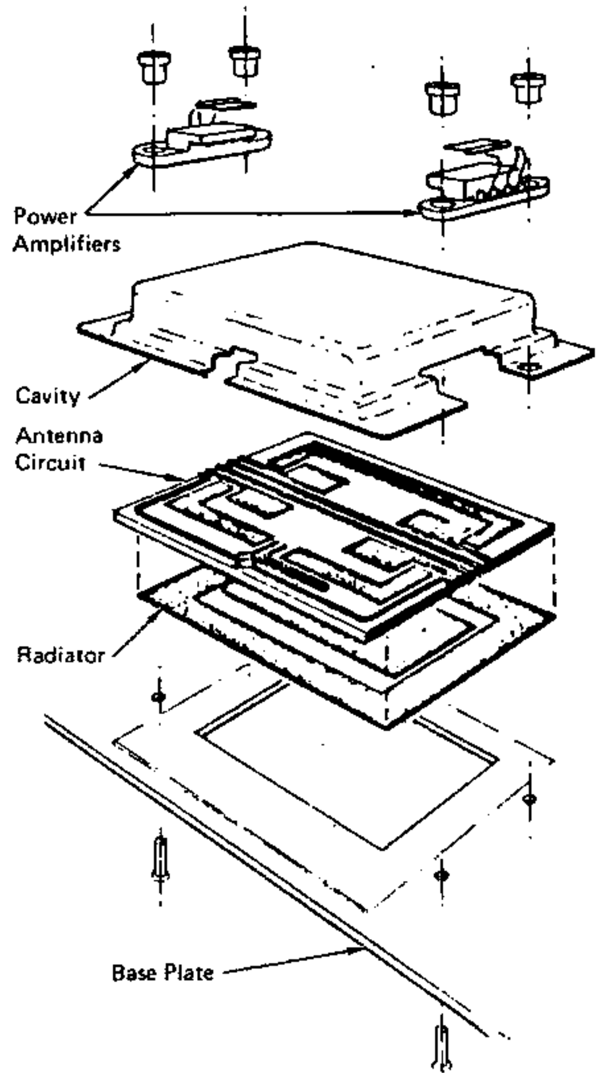
Figure 8. Solid-State Combiner Radiator Module
