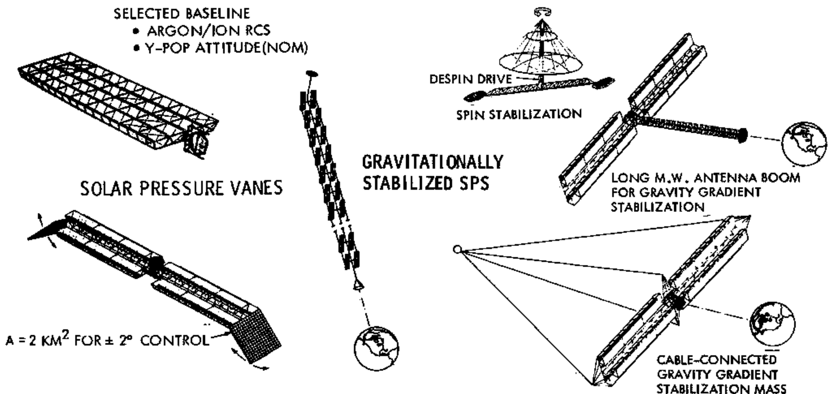
Figure 2. Attitude Control Concepts
