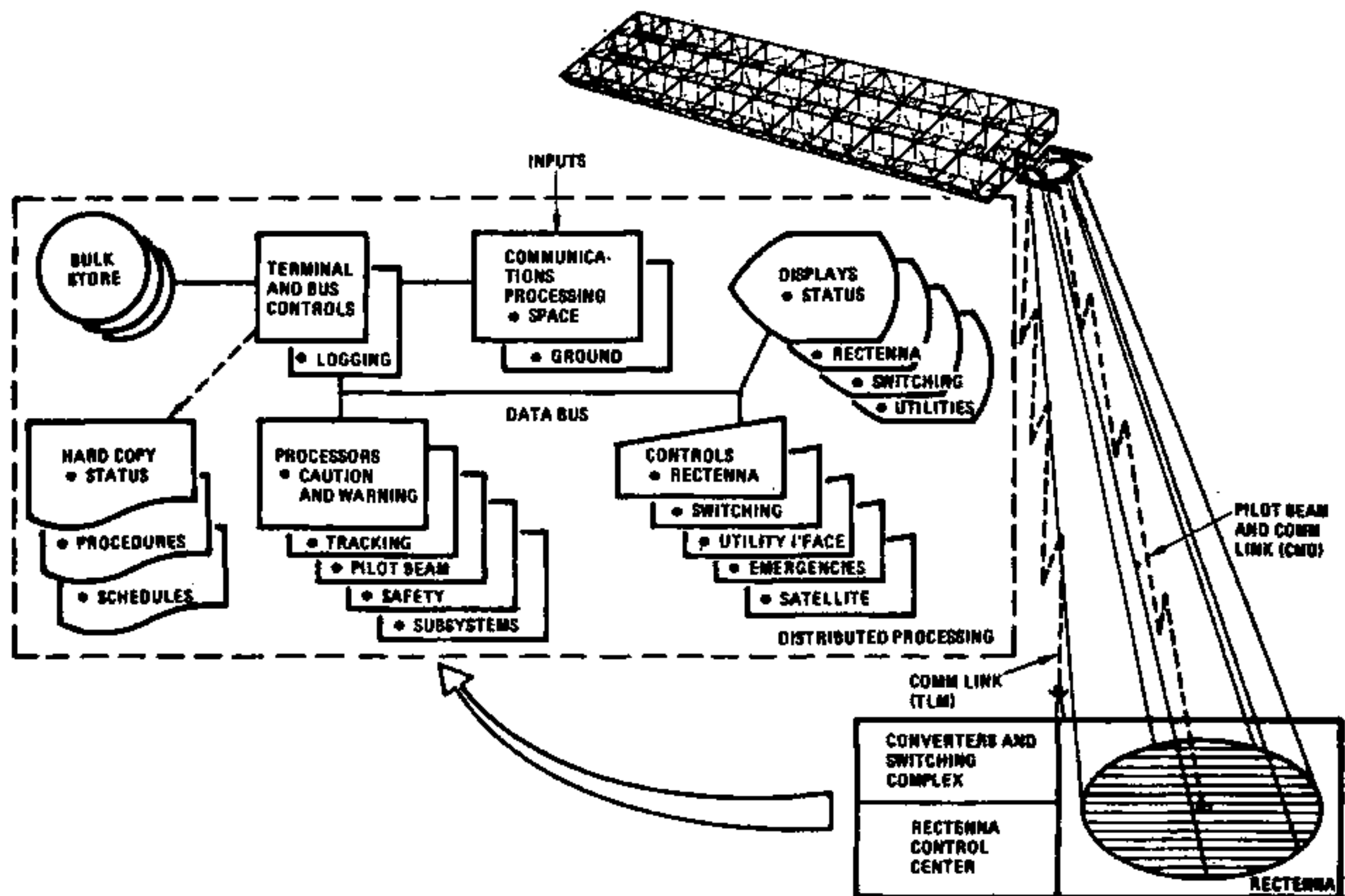
Figure 4. Rectenna Control Center Concept
