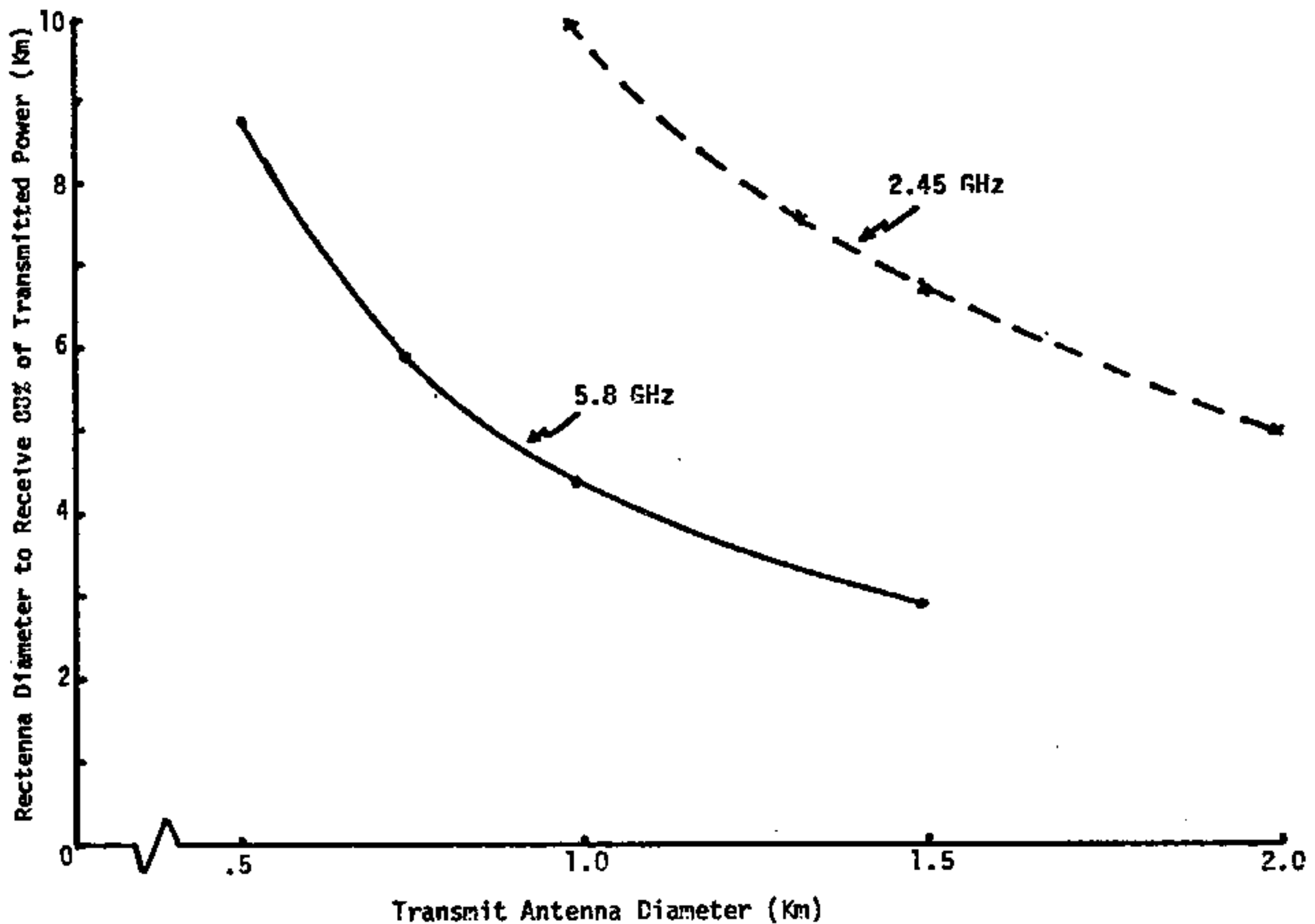
Figure 1. Antenna/Rectenna Sizing Summary
