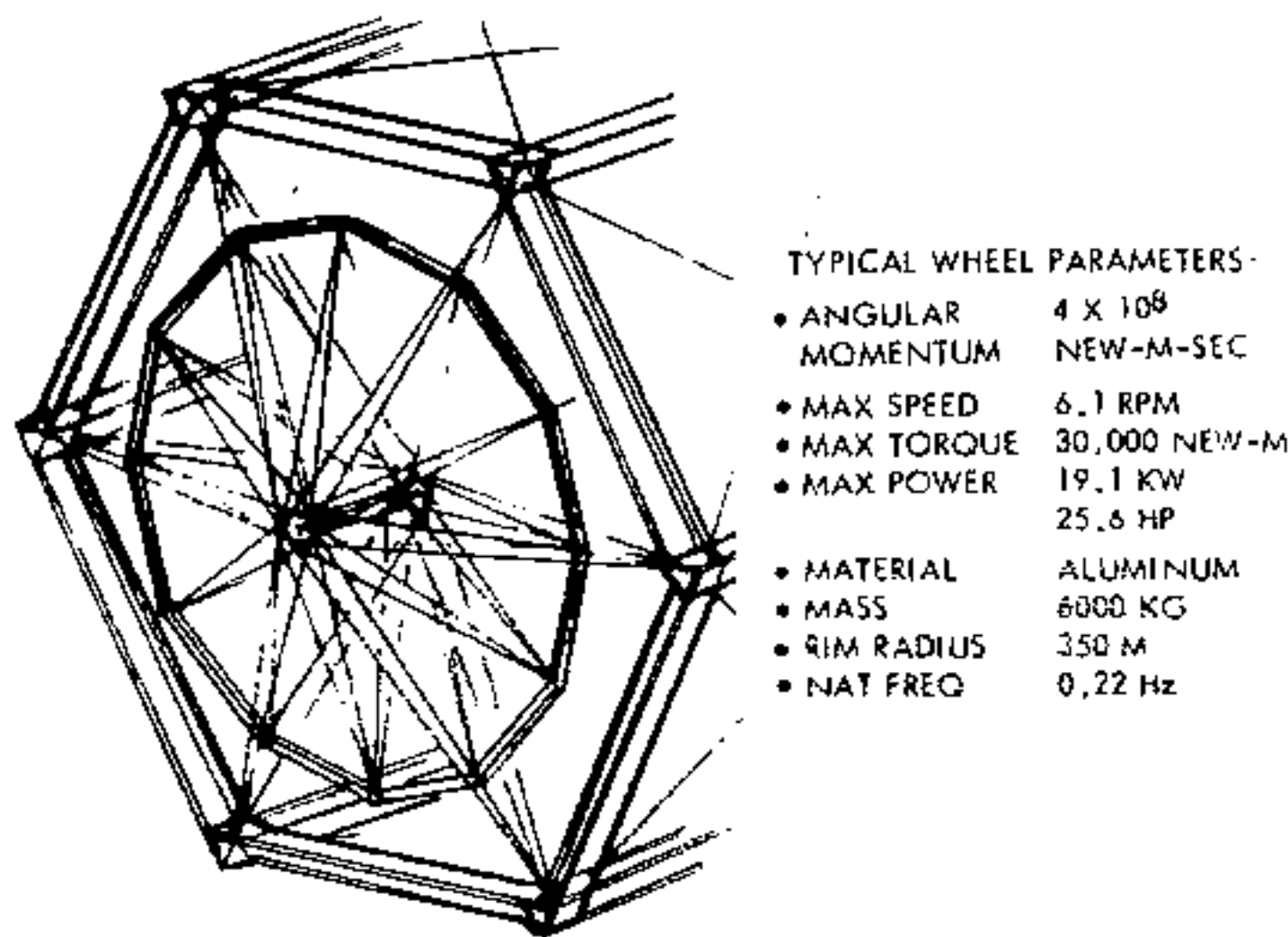
Figure 3. Erectable Momentum Wheel Conceptual Design
