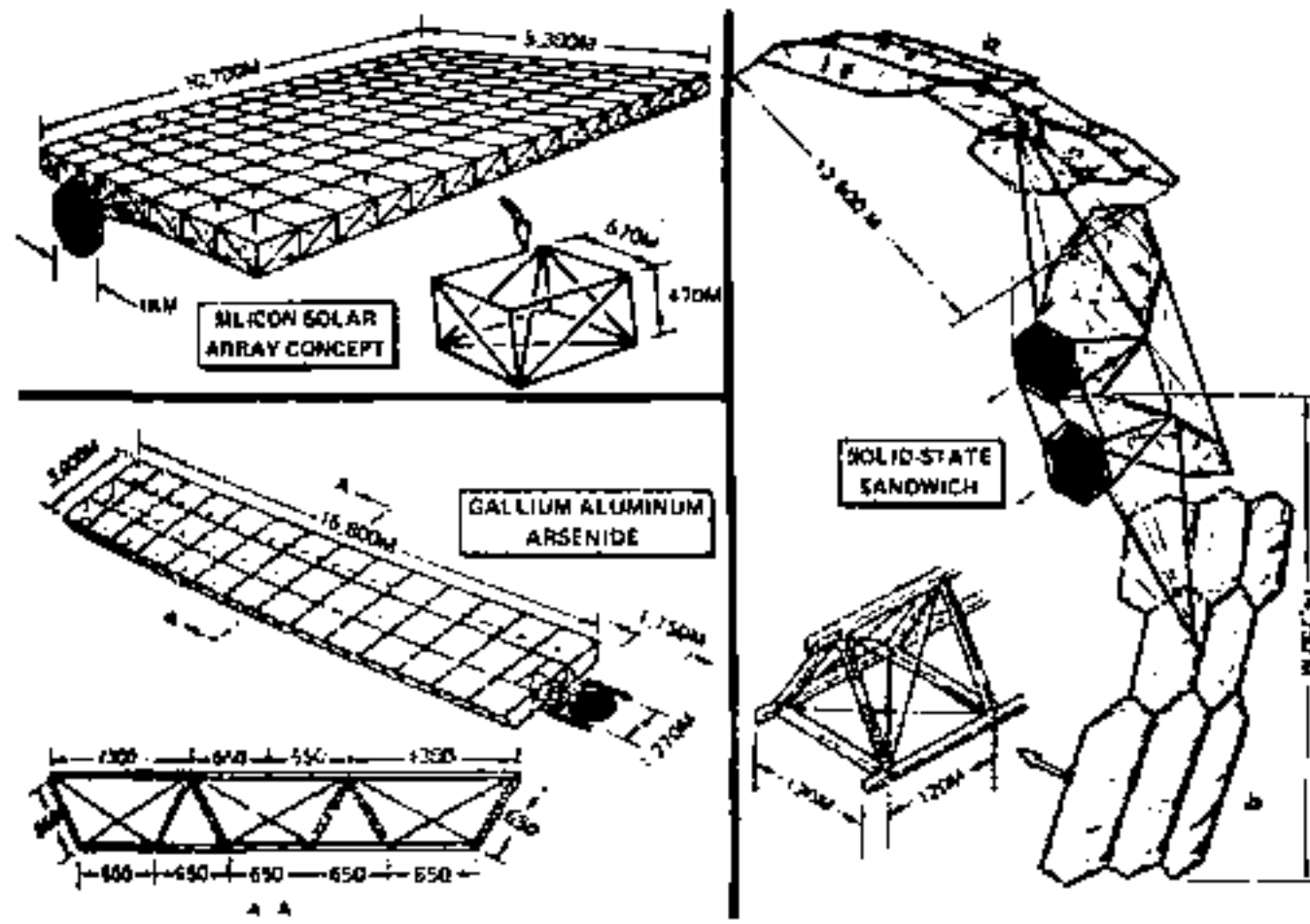
Figure 1. SPS Current Configurations
