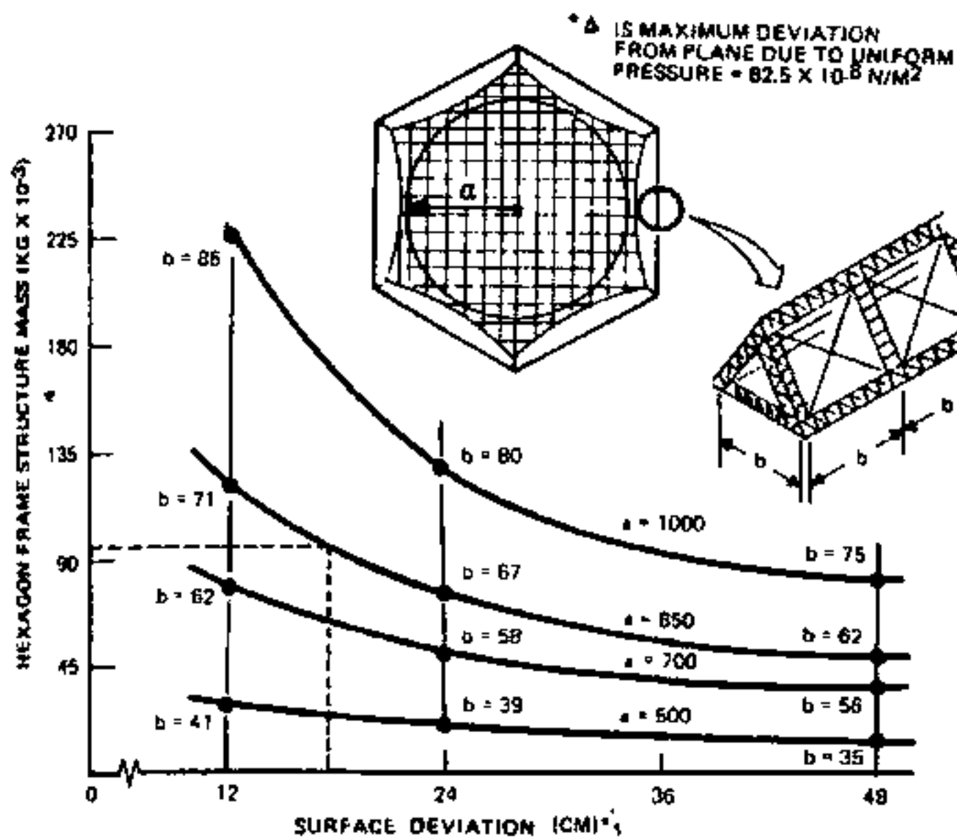
Figure 5. Hexagon Frame Mass Versus Surface Deviation (cm)
