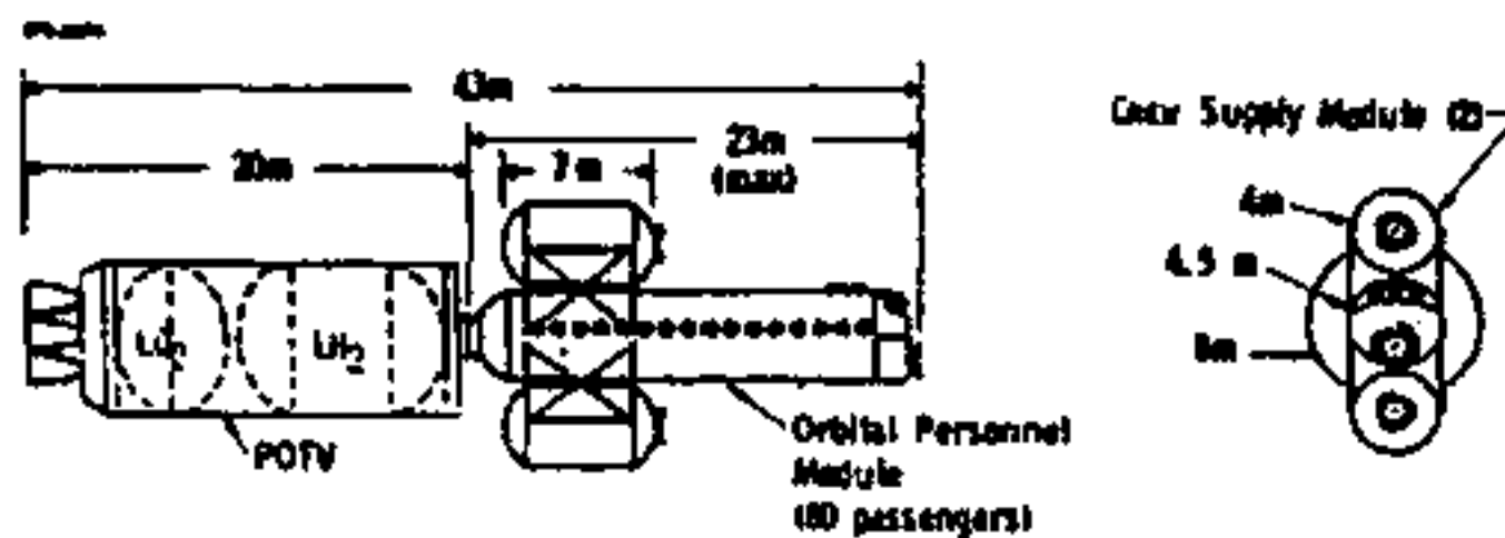
Figure 2- ORBITAL PERSONNEL MODULE
