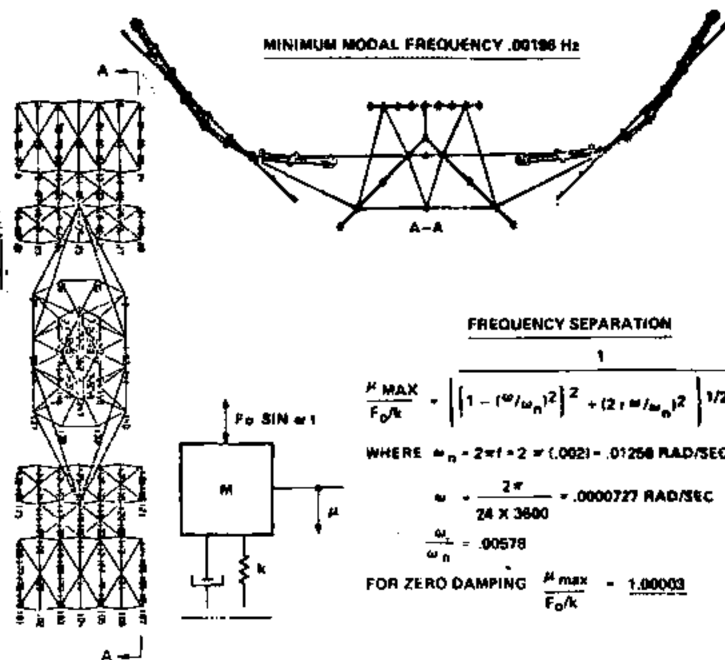
Figure 6. Minimum Modal Frequency Implications
