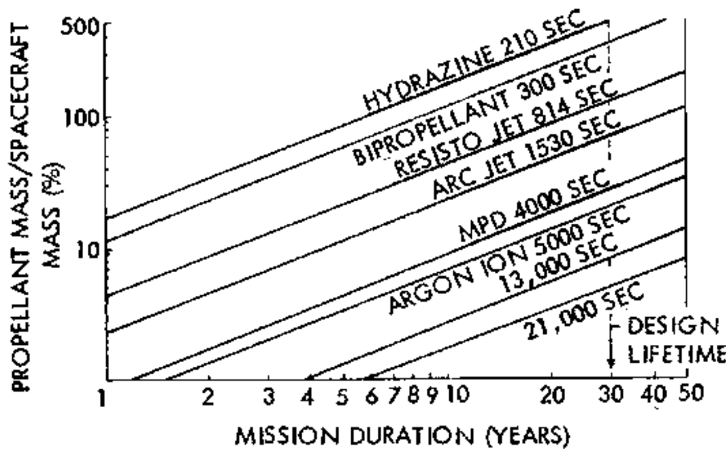
Figure 4. Propellant Requirements for Various RCS Propulsion Types
