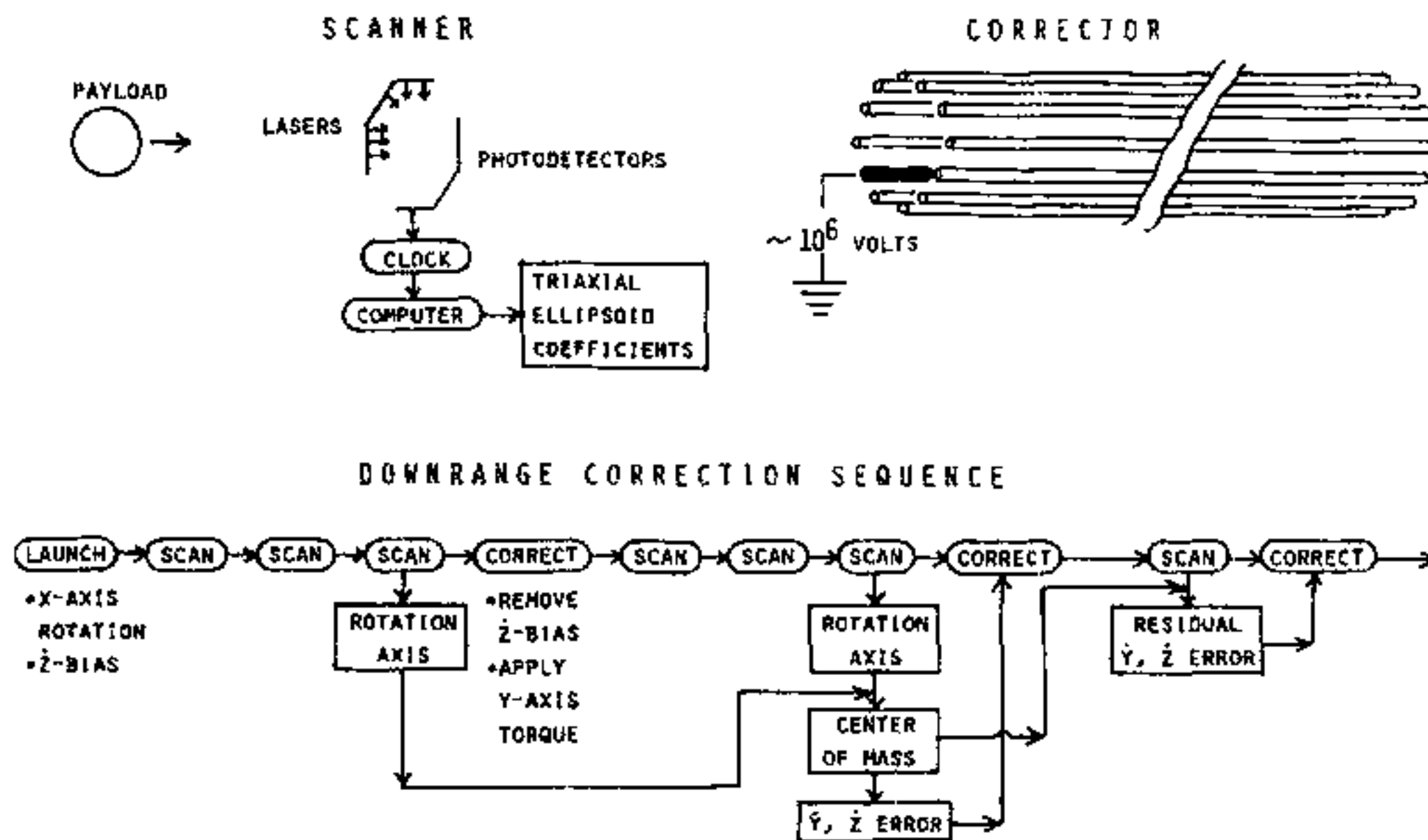
Figure 6. Downrange correction. Scanner employs six lasers plus timed photodetectors to determine payload location, dimensions, and orientation. Corrector charges a selected conductor within an array for electrostatic deflection of payload; payload is electrically neutral but conductor induces a charge redistribution. Correction sequence determines initial rotation axis, applies a lateral torque to payload, then redetermines rotation axis, thus yielding payload mass center location. Thereafter observed payload lateral position errors are interpreted as due to lateral velocity components of center of mass, which are electrostatically corrected. Final scan/correction steps occur atop a mountain some 75 kilometers (30 seconds flight time) downrange from launch site.
