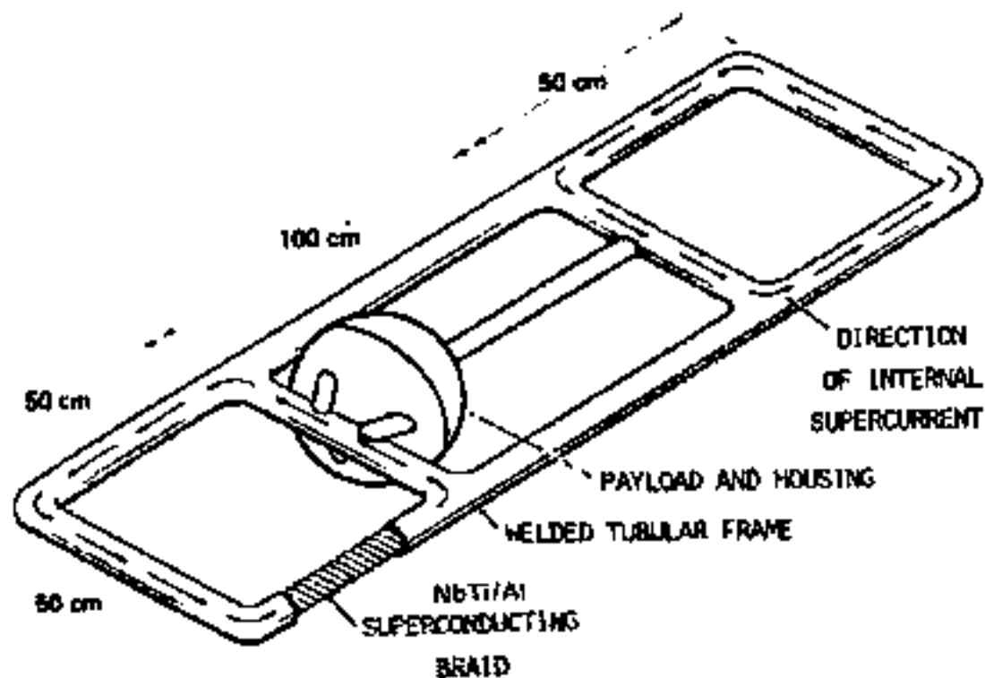
Figure 2. Mass-driver bucket. Frame is cut away to show superconducting braid. Note payload constraint/release system. (Modified from Chilton et. al., op. cit., p. 50)
