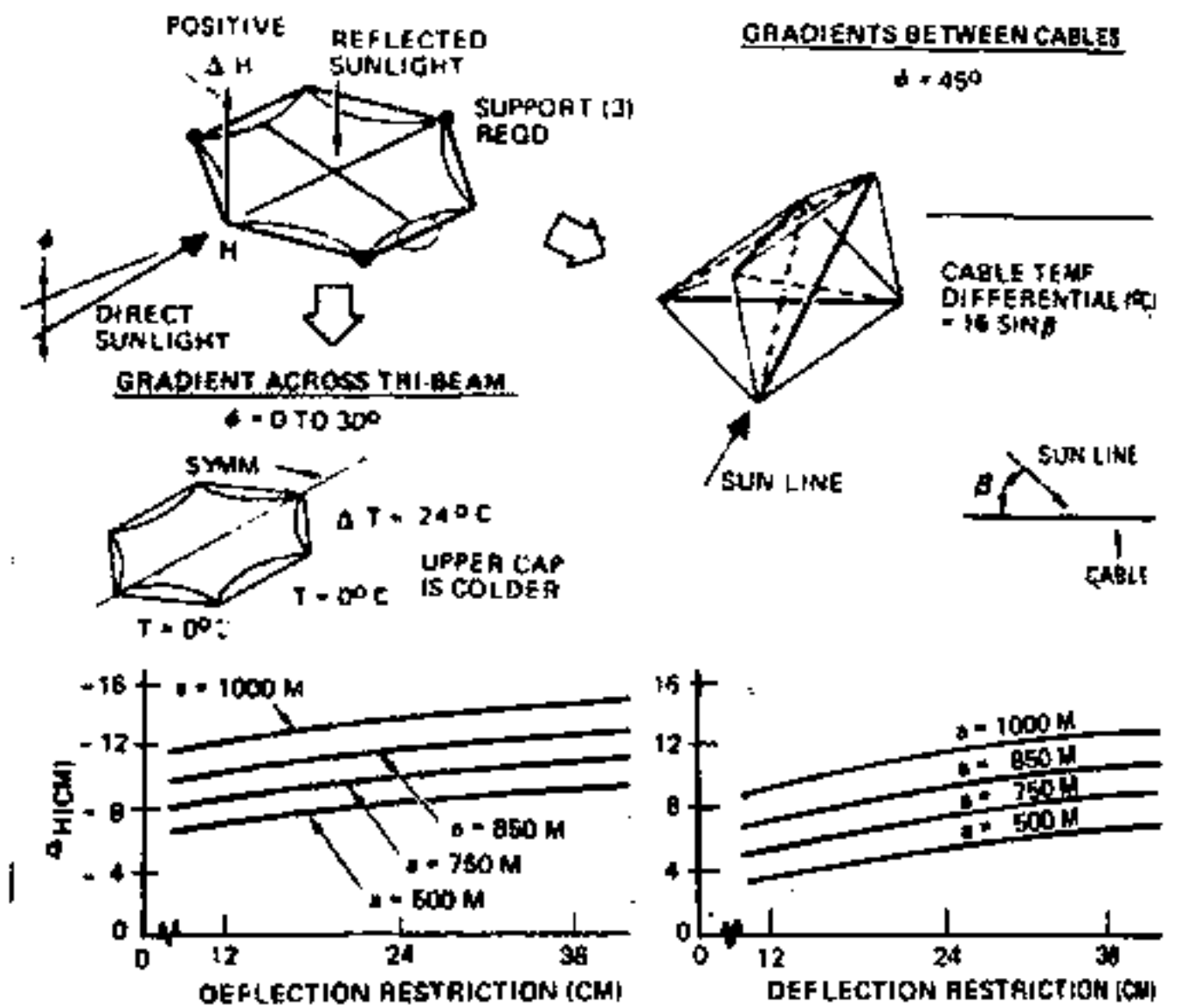
Figure 4. Frame Thermal Deflections
