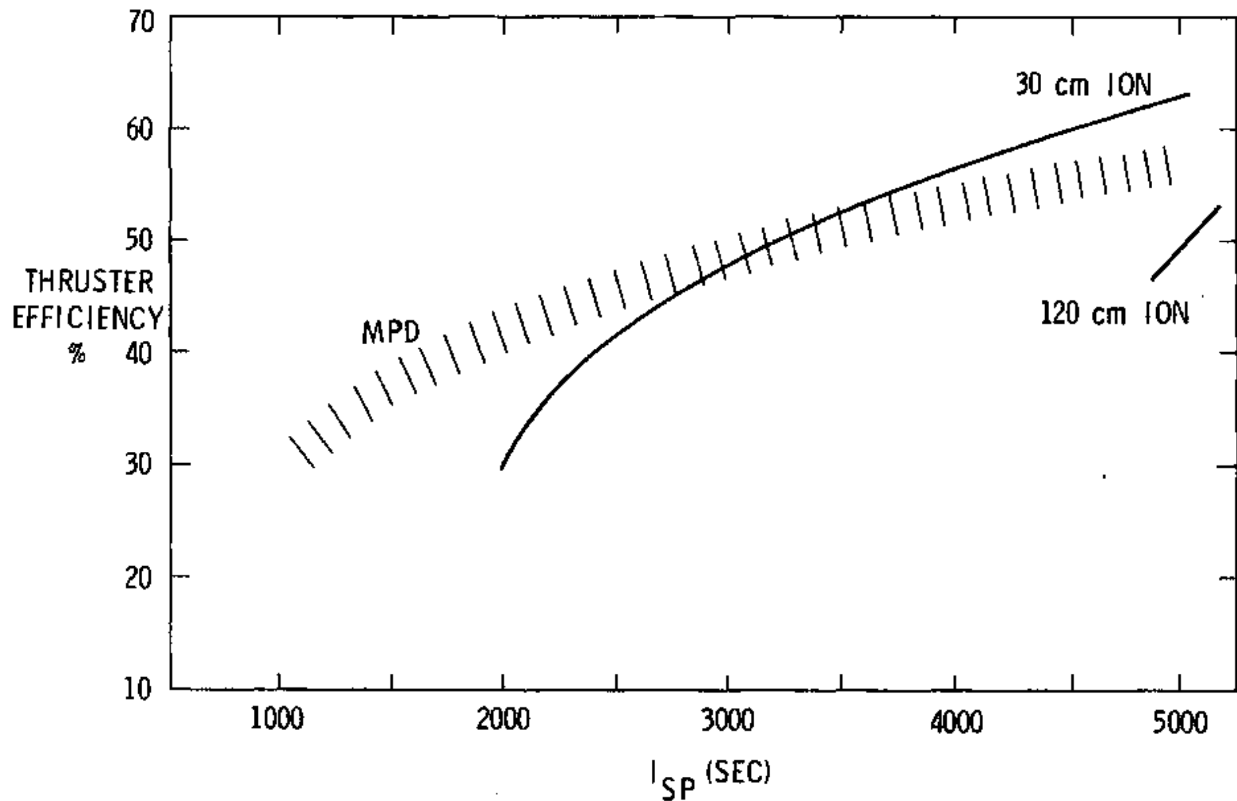
Fig. 1. Comparison of MPD and ion thruster efficiency with argon.
