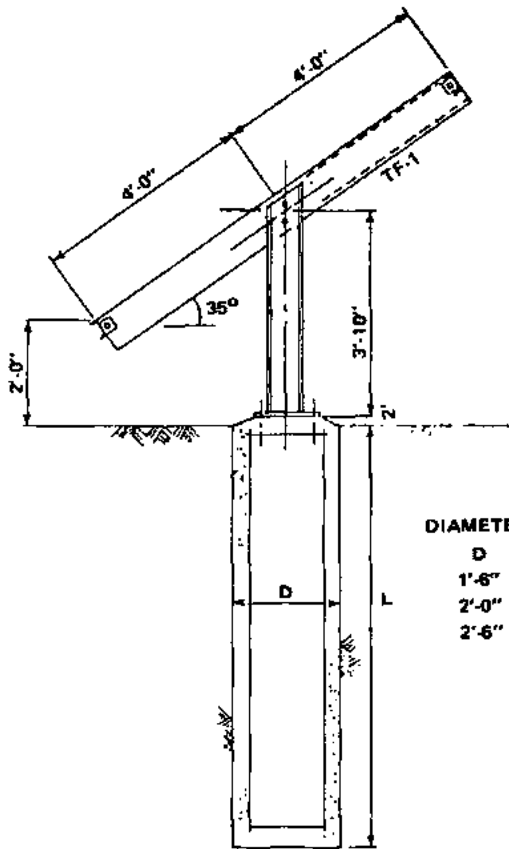
VERTICAL CAISSON F-3, 8' x 20' ARRAYS
