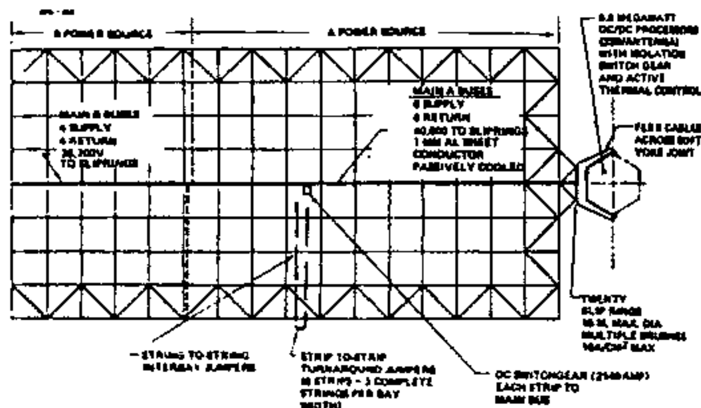
Figure 3- MULTIPLE BUS SPS POWER DISTRIBUTION
