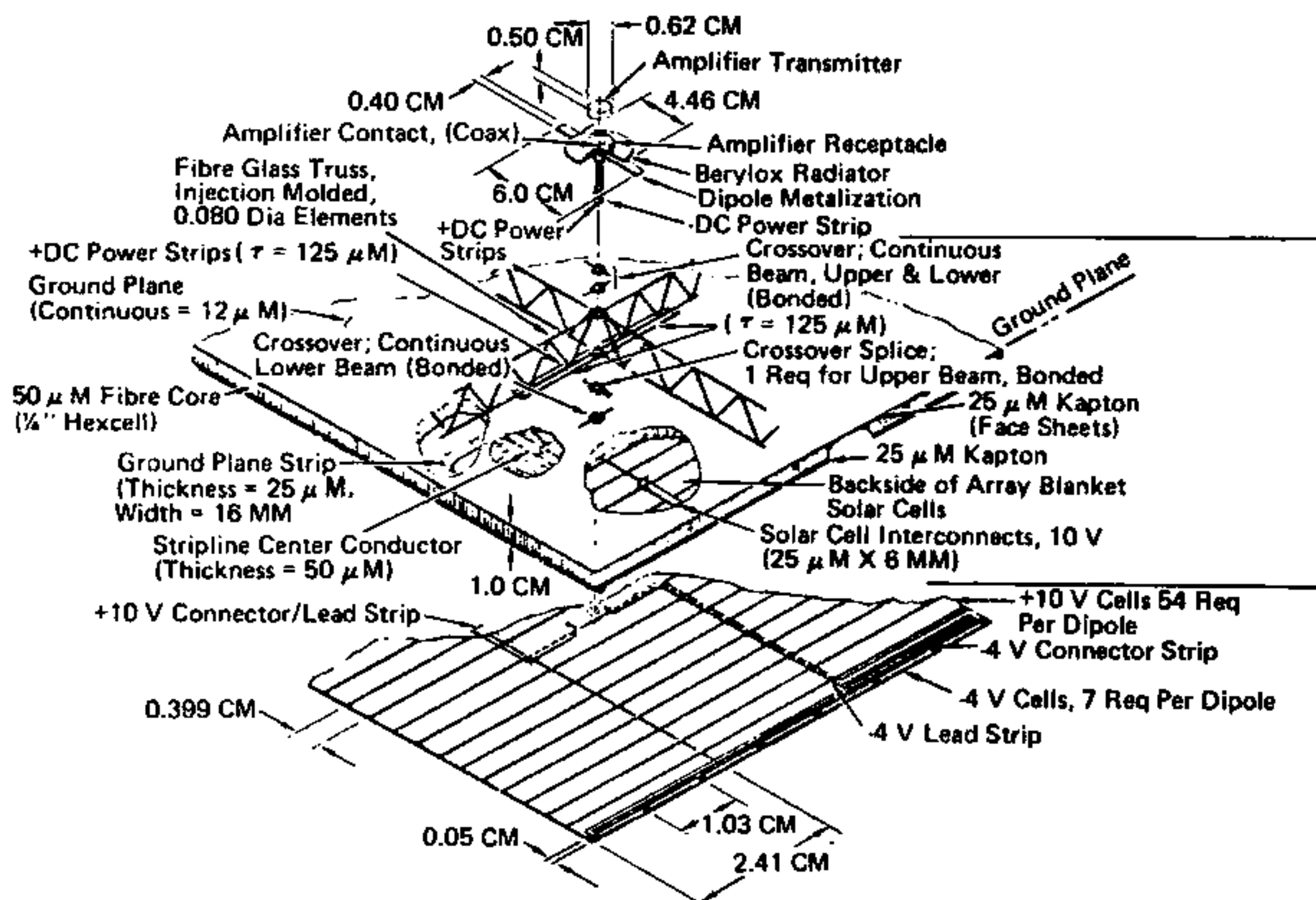
Figure 7. Sandwich Antenna Dipole
