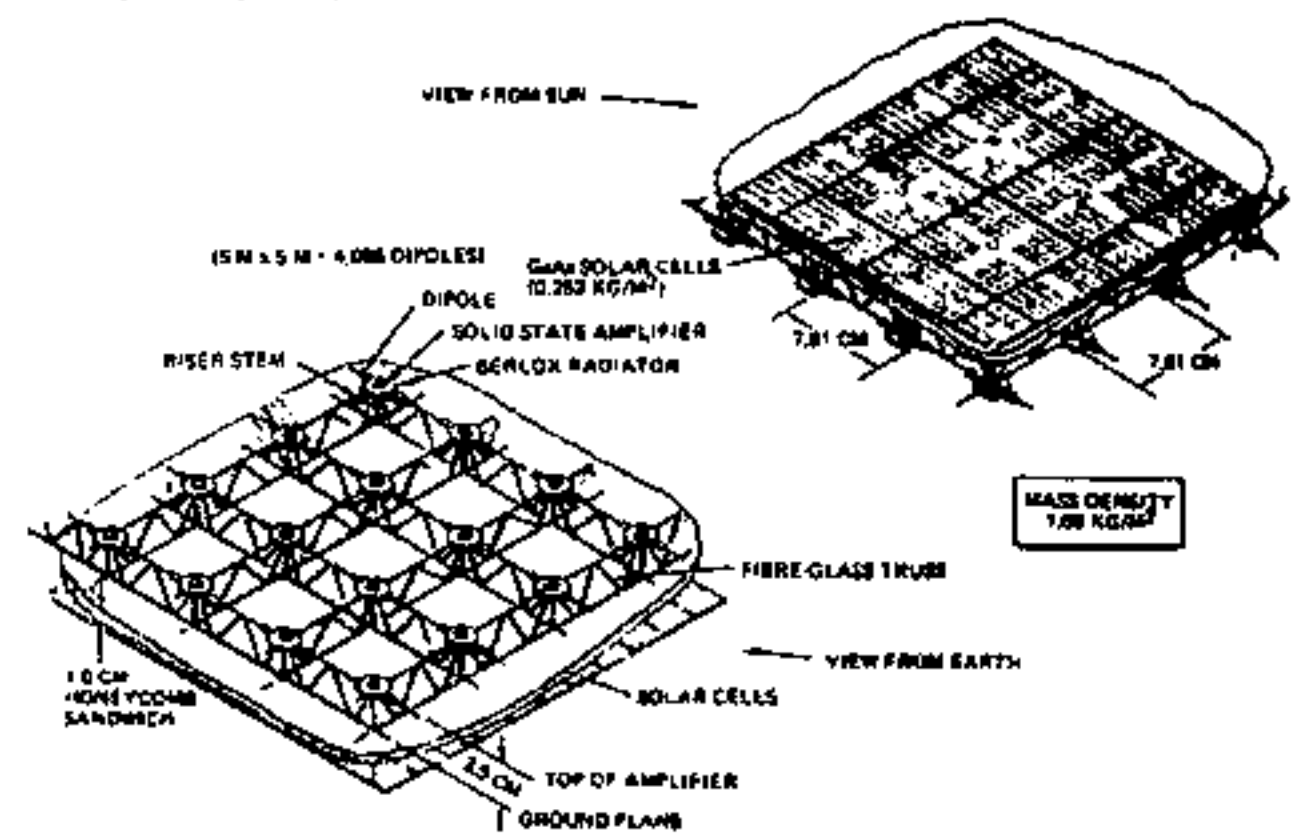
Figure 3. Solid-State Sandwich Design
