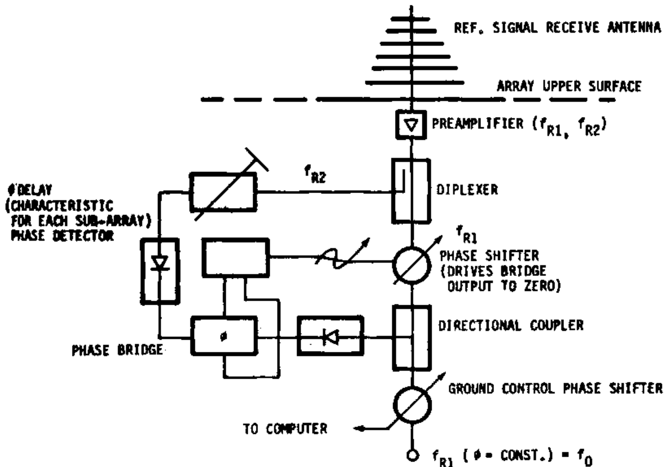
FIGURE 4. REFERENCE SIGNAL CONTROL LOOP
