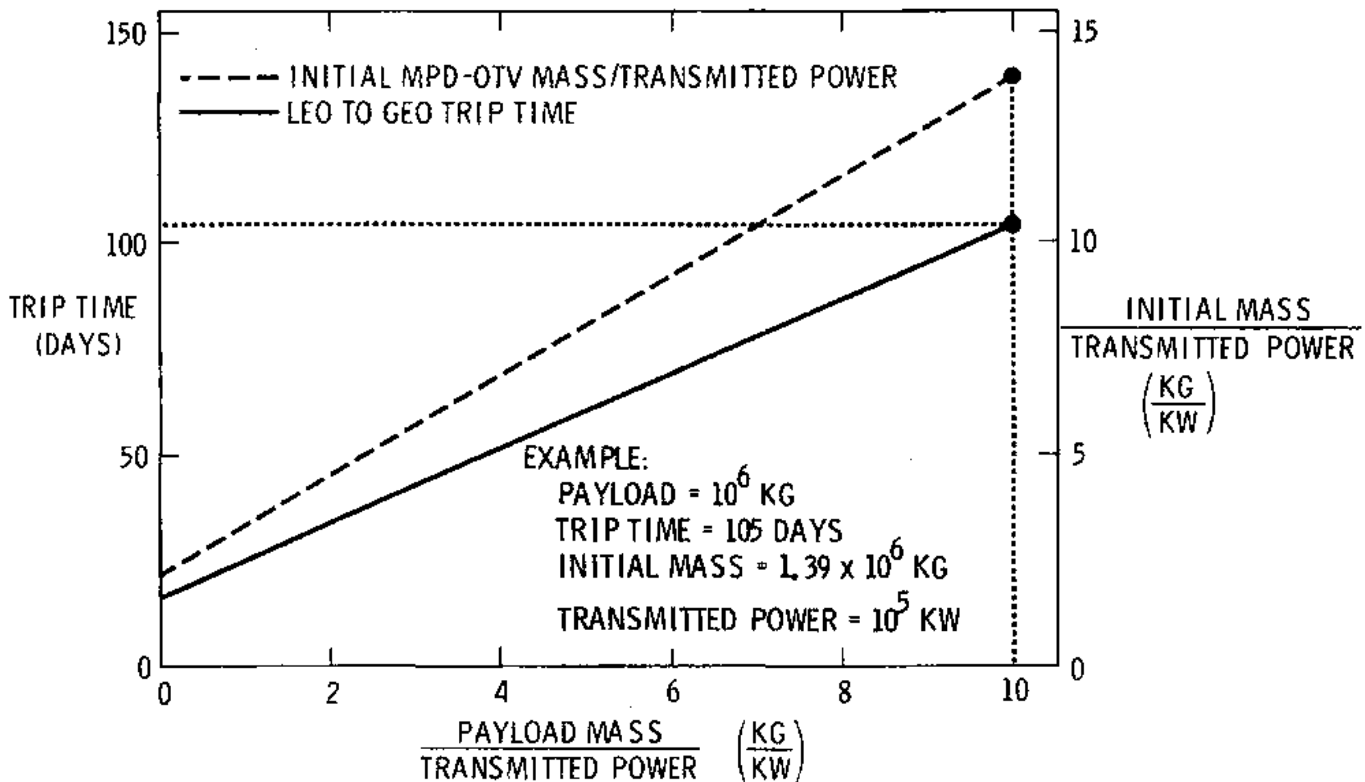
Fig. 4. Mission performance for microwave powered MPD-COTV.
