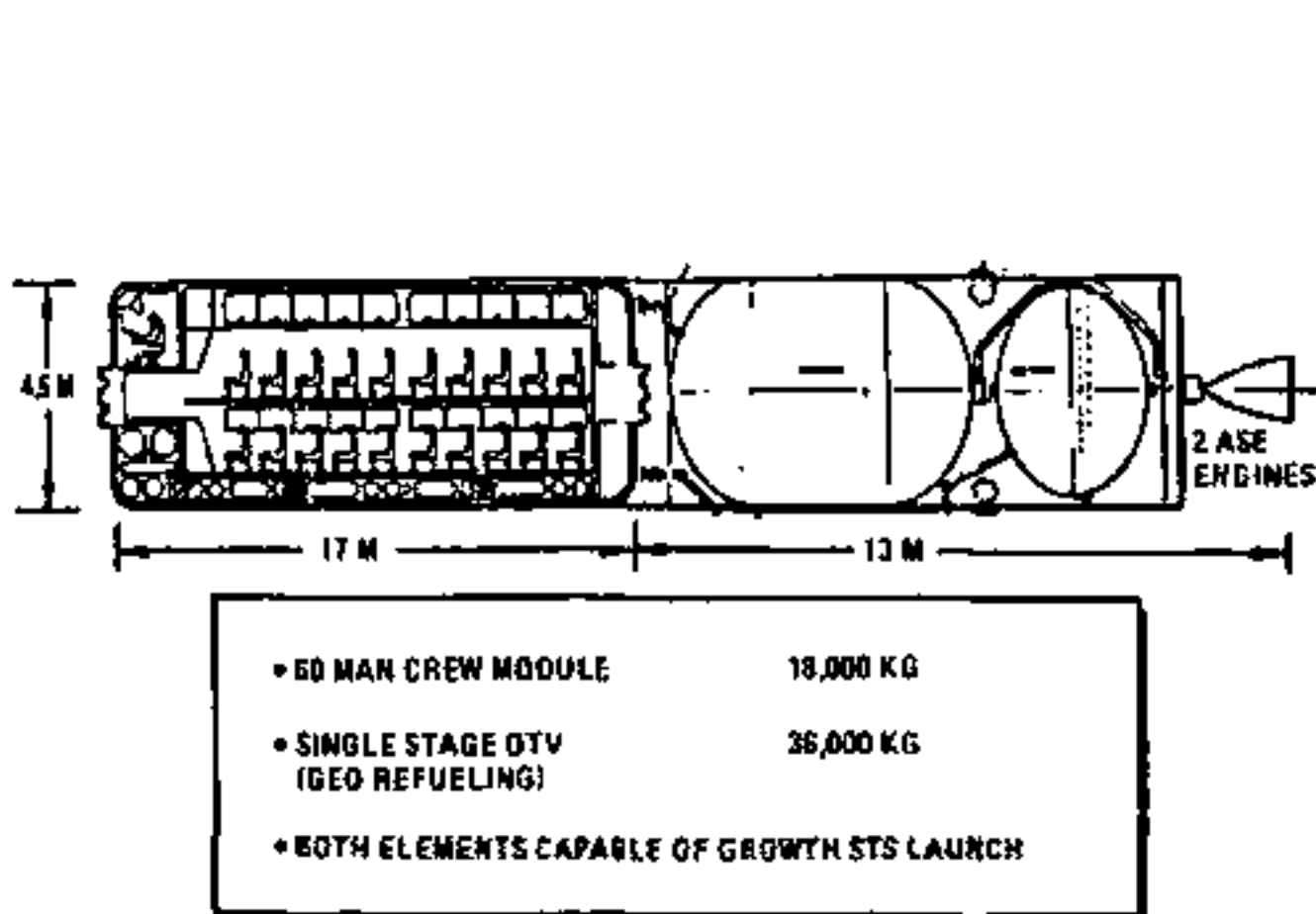
Figure 3. Personnel Orbital Transfer Vehicle
