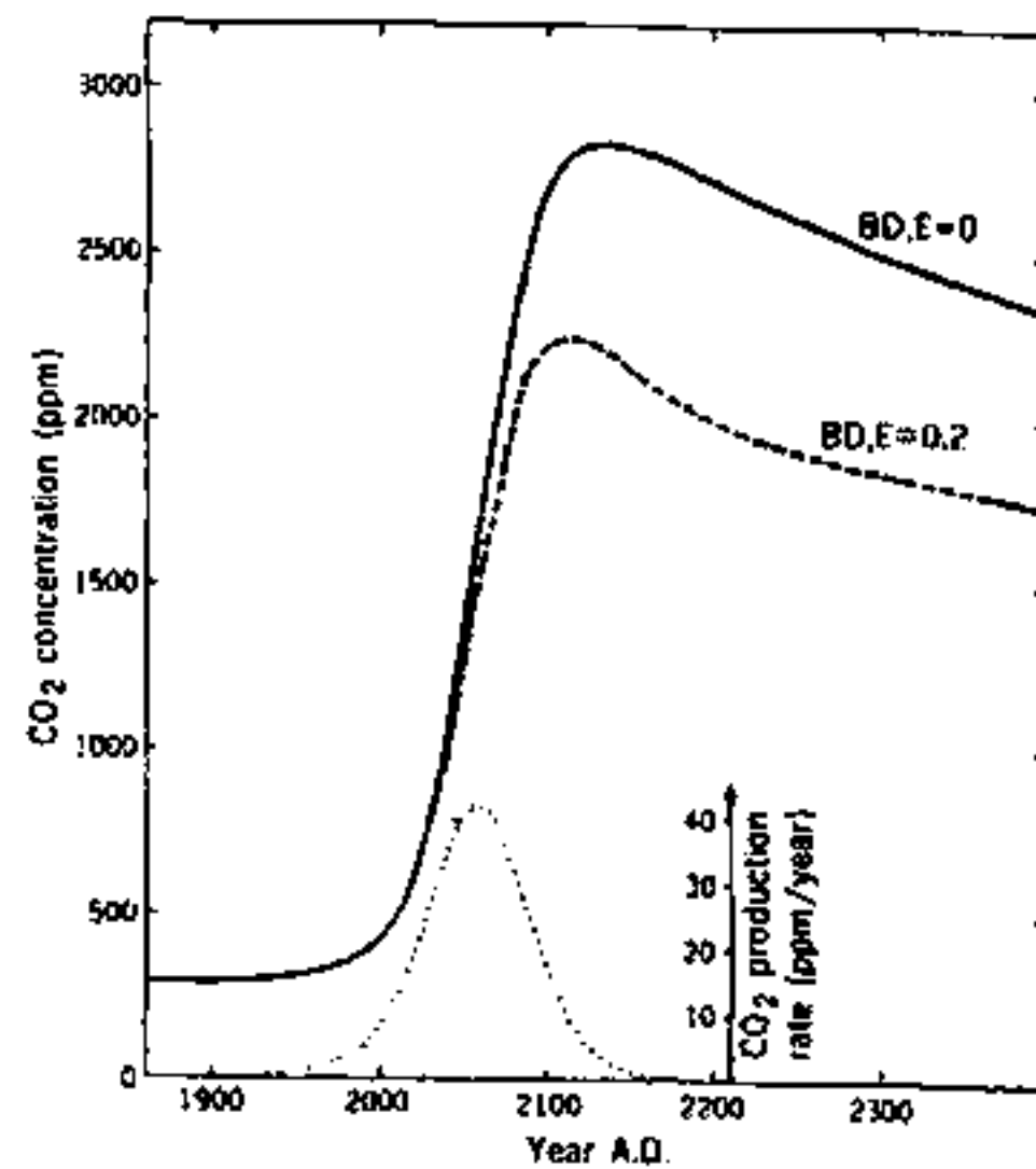
Figure 6. Predictions for the case in which all recoverable fossil fuels are burned. Lowermost curve shows resulting \text{CO}_2 production rate, if fossil-fuel use grows at 5% per year. The two \text{CO}_2 concentration curves reflect two models used; the dashed curve is regarded as less probable. (After Siegenthaler and Oeschger, op. cit. )
