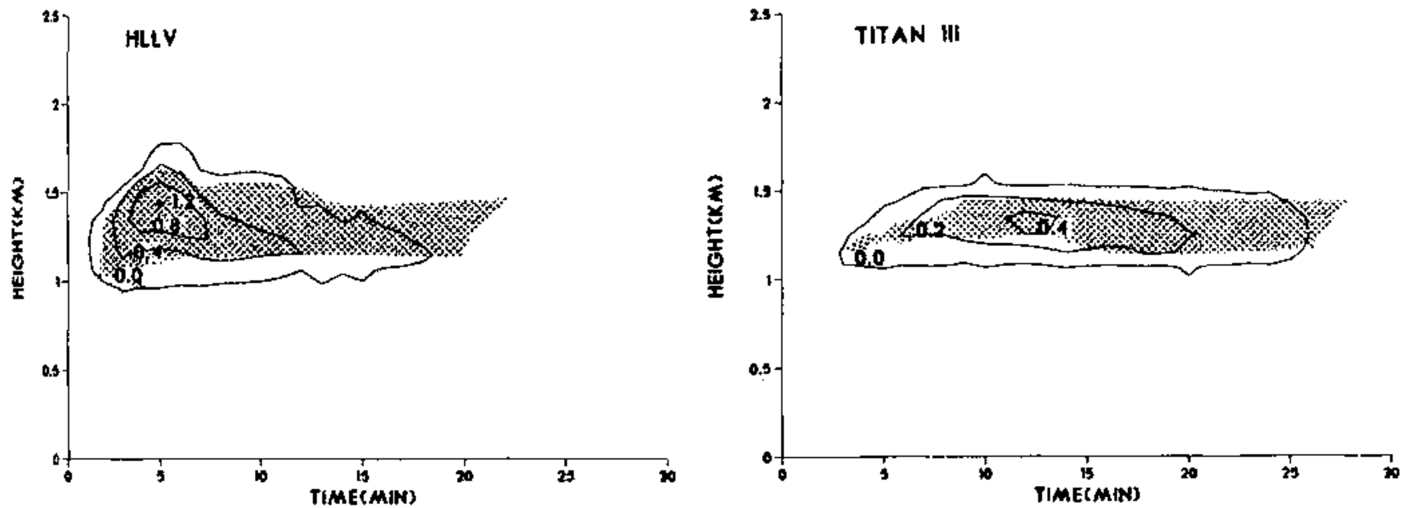
Fig. 3. Comparison of predicted mean cloud liquid water content (g/kg) between HLLV and Titan III clouds. Shaded areas indicate saturation regions.
