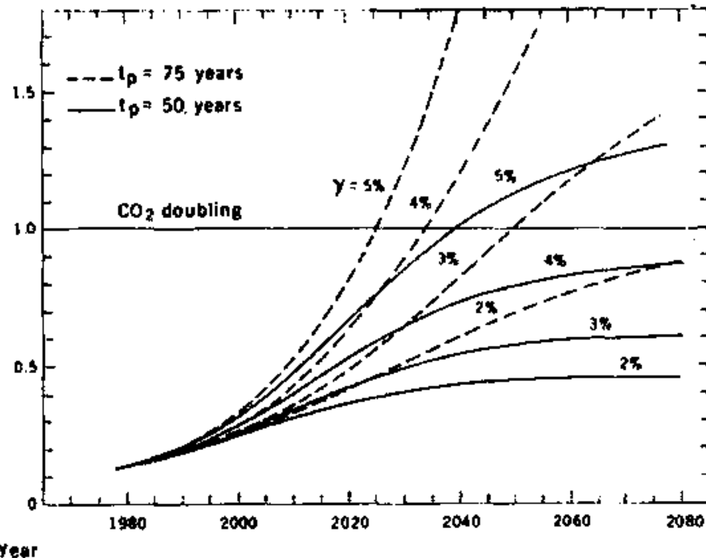
Figure 7. Left, fractional growth of atmospheric \text{CO}_2 concentration G above the preindustrial value for various initiation dates t_0 relative to 1975 of noncarbon-based energy, with world energy growth rate of 3% per year, and a market penetration time of 50 years (time for the new energy source to advance from 1% to 50% share of market). Right, fractional growth of atmospheric \text{CO}_2 for various annual world energy growth rates \gamma , and two market penetration times t_p . The 1% market share of the noncarbon-based fuel is taken to have occurred in 1965 ( t_0 = -10 years). (After Laurmann, Science 205, 1979, p. 896)
