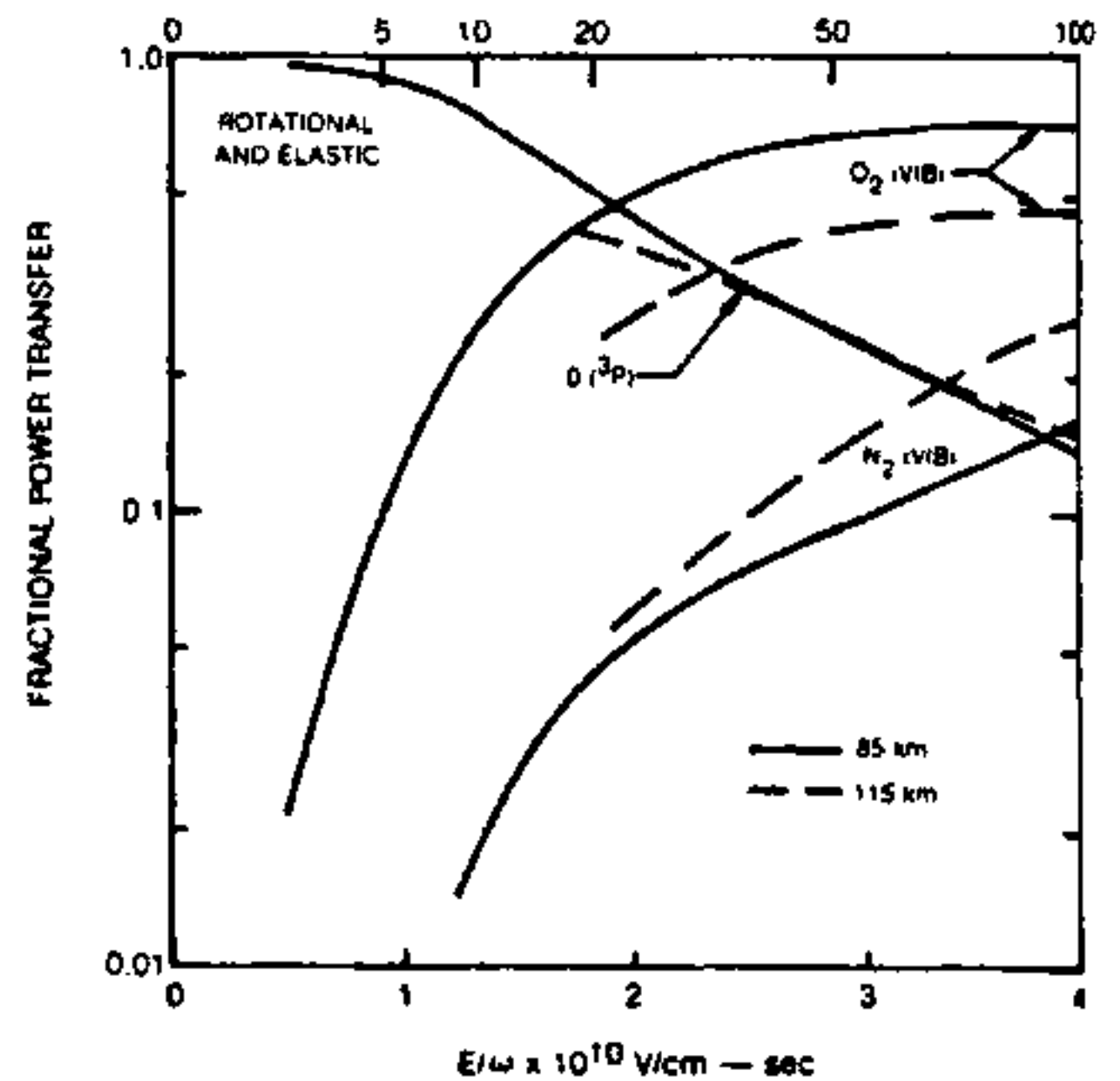
Fig. 2b Electron Cooling Mechanisms
