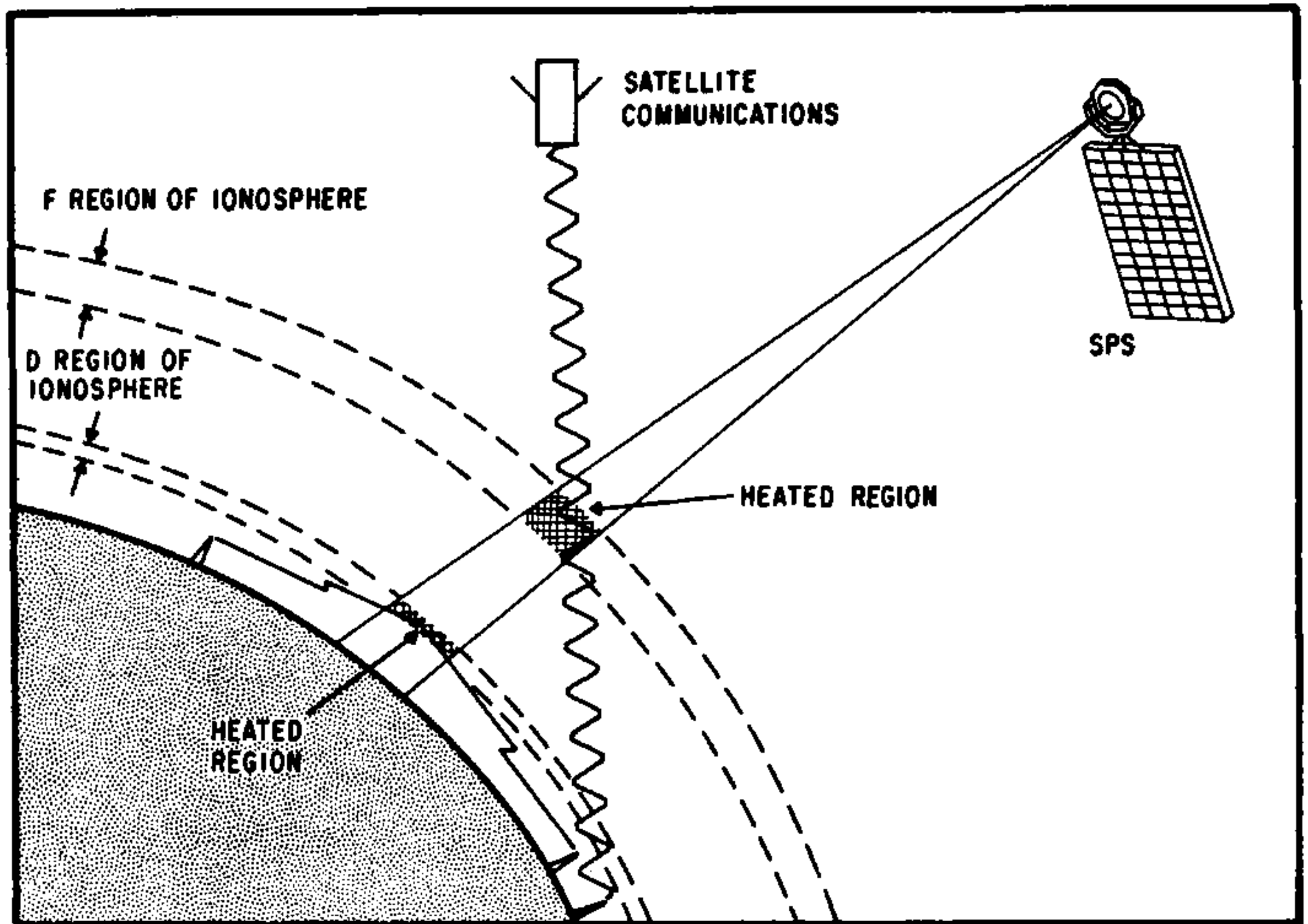
Fig. 4. Examples of SPS Microwave Transmission Effects on the Ionosphere and Telecommunication Systems
