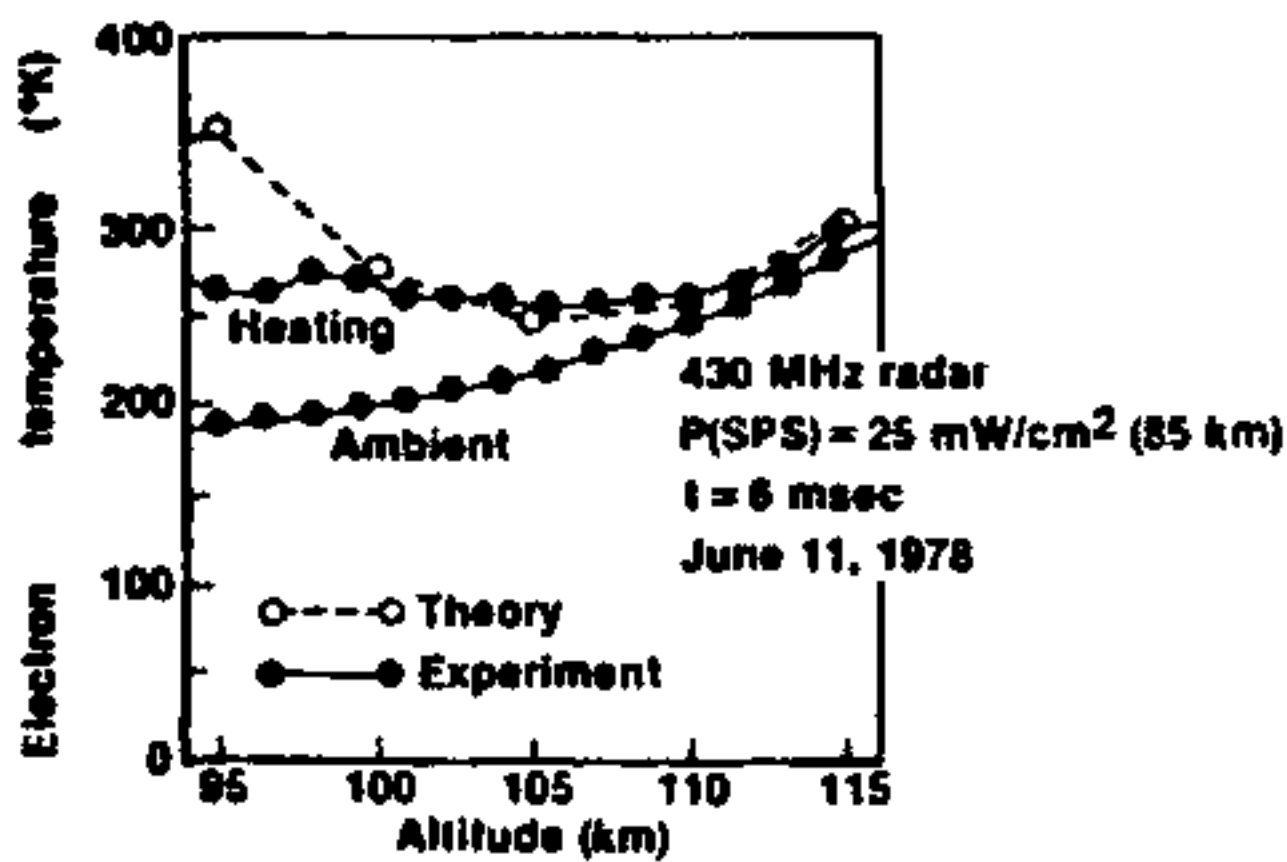
Fig. 3 Arecibo Electron Heating Observations
