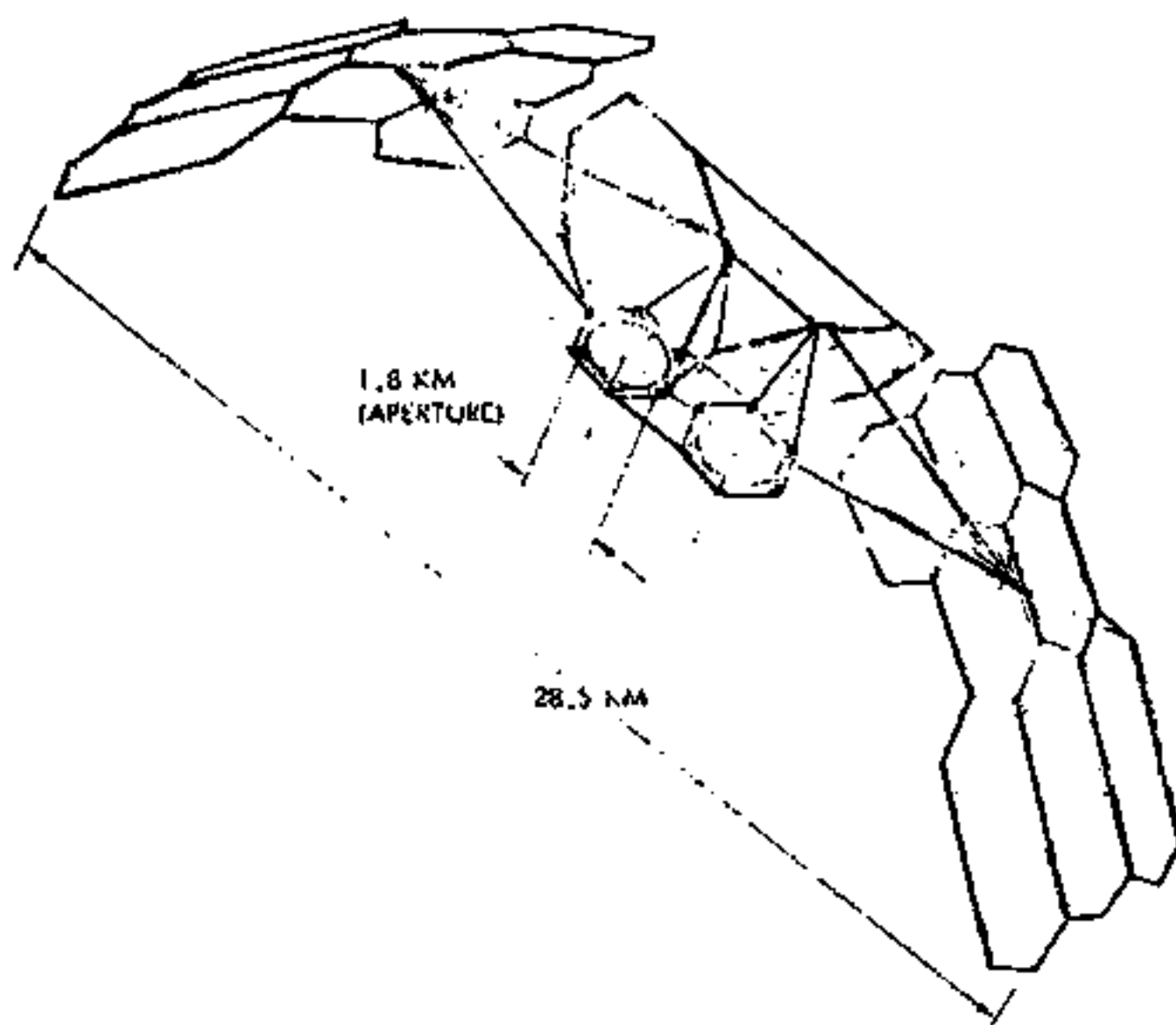
Figure 2. Solid-State Sandwich Satellite Concept
