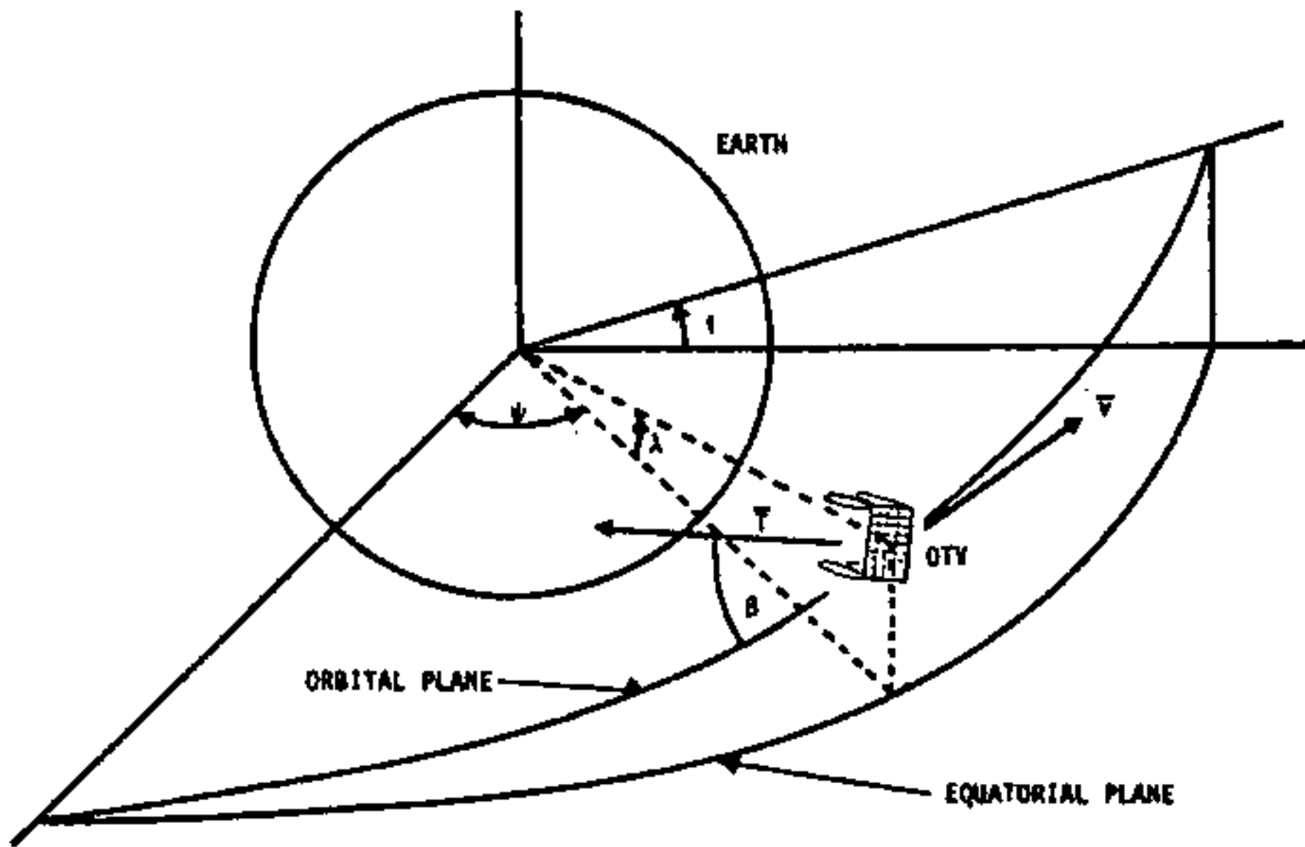
FIGURE 1. ORBITAL GEOMETRY AND THRUSTER EXHAUST FOR OTV
