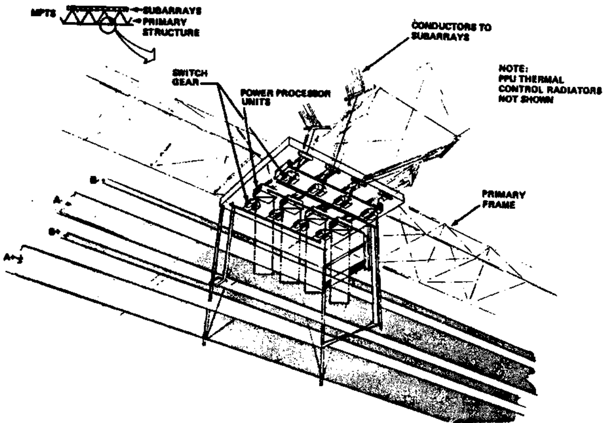
Figure 6- MPTS POWER PROCESSING SUBSTATION
