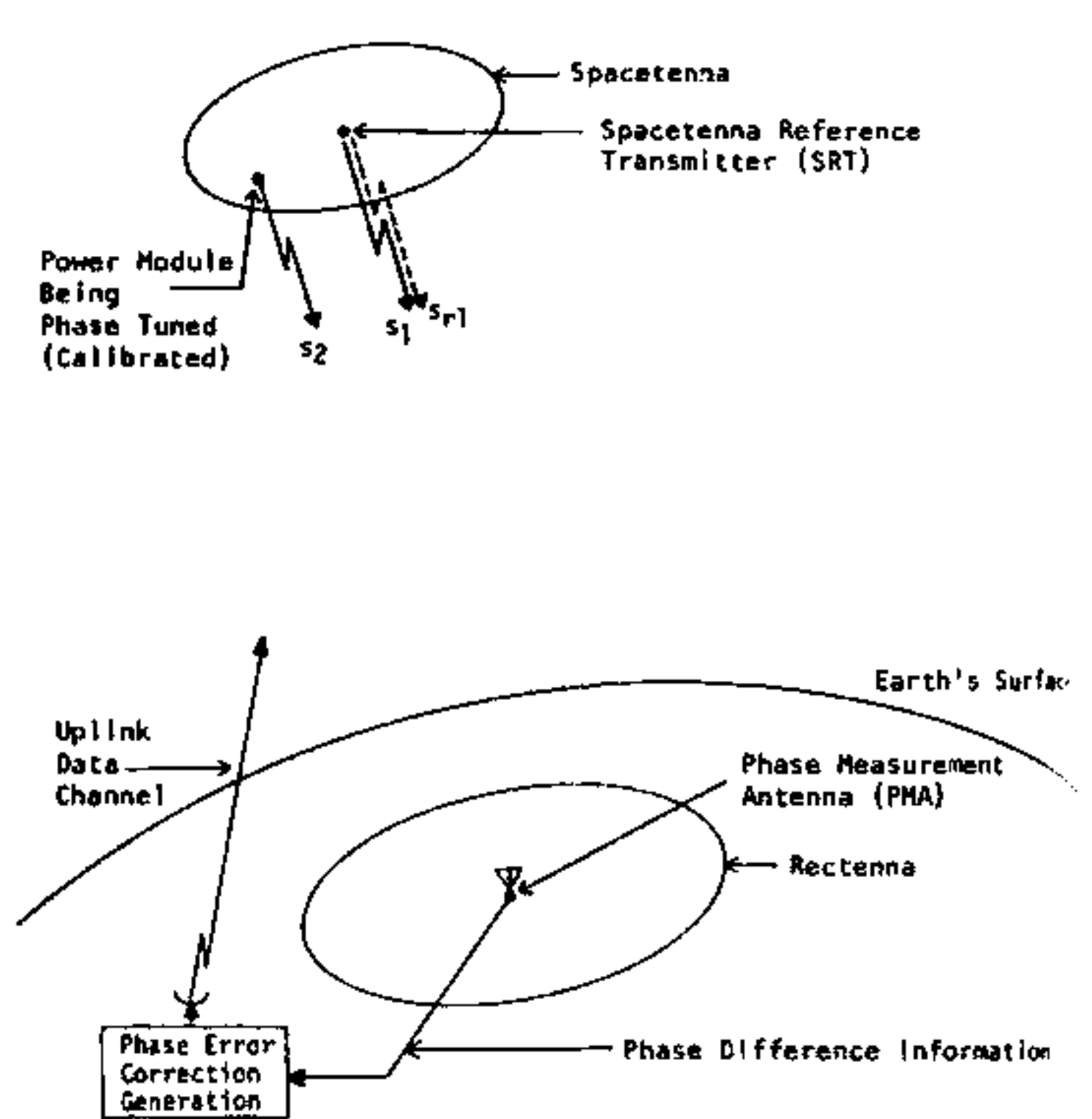
Pictorial representation of relationship between Spacetenna signals and ground instrumentation. FIGURE 2 INTERFEROMETRIC PHASE CONTROL
