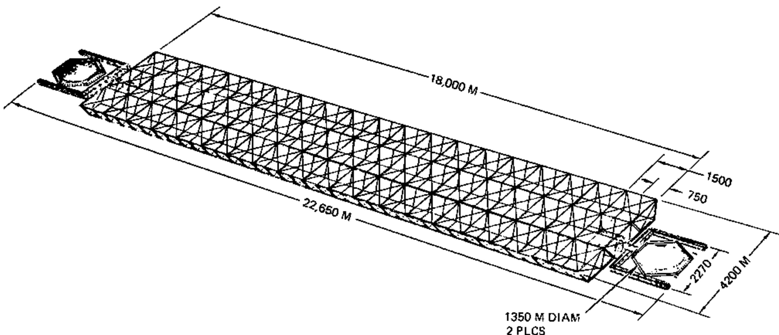
Figure 1 Solid-State End-Mounted Antenna Satellite Concept
