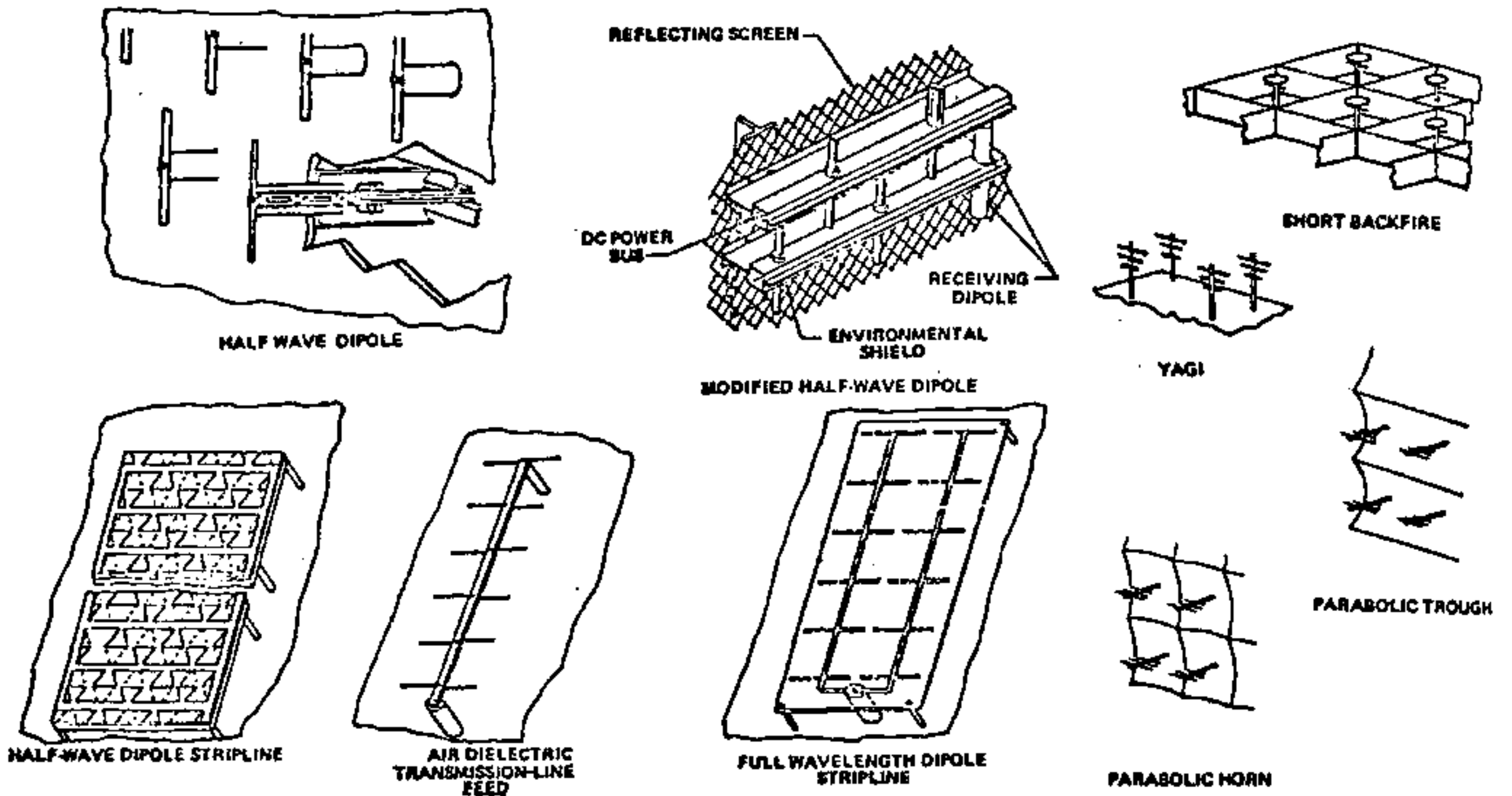
Figure 2: Rectenna Receiving Element Options
