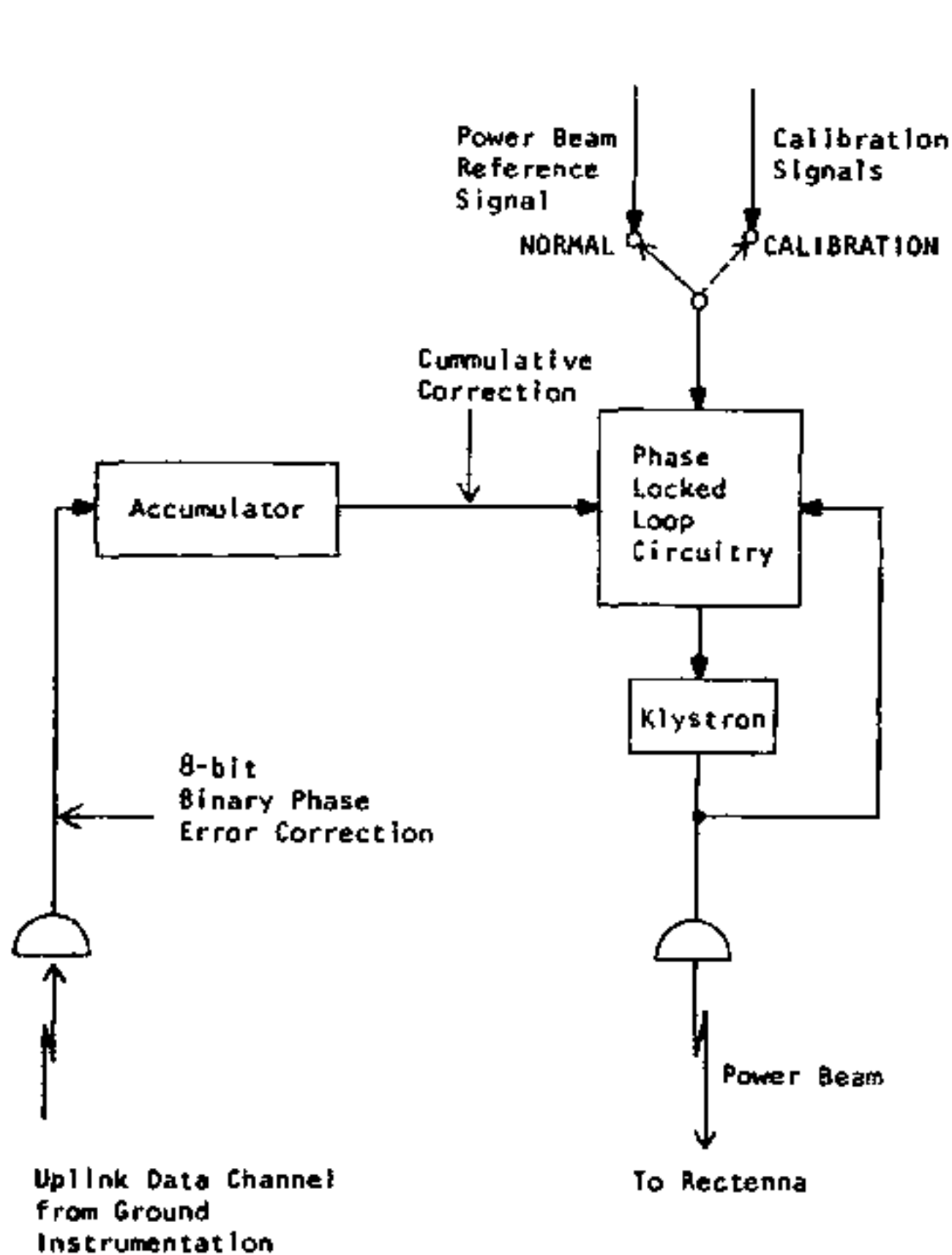
FIGURE 1 POWER MODULE PHASE CONTROL CIRCUITRY
