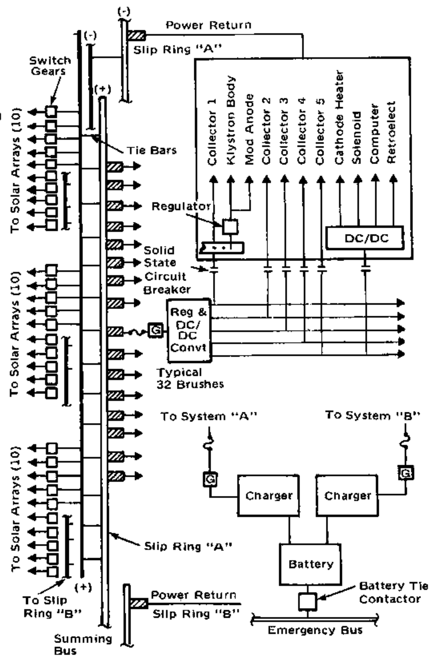
Figure 1. SPS Reference Configuration (GaAs Cells, CR=2)
