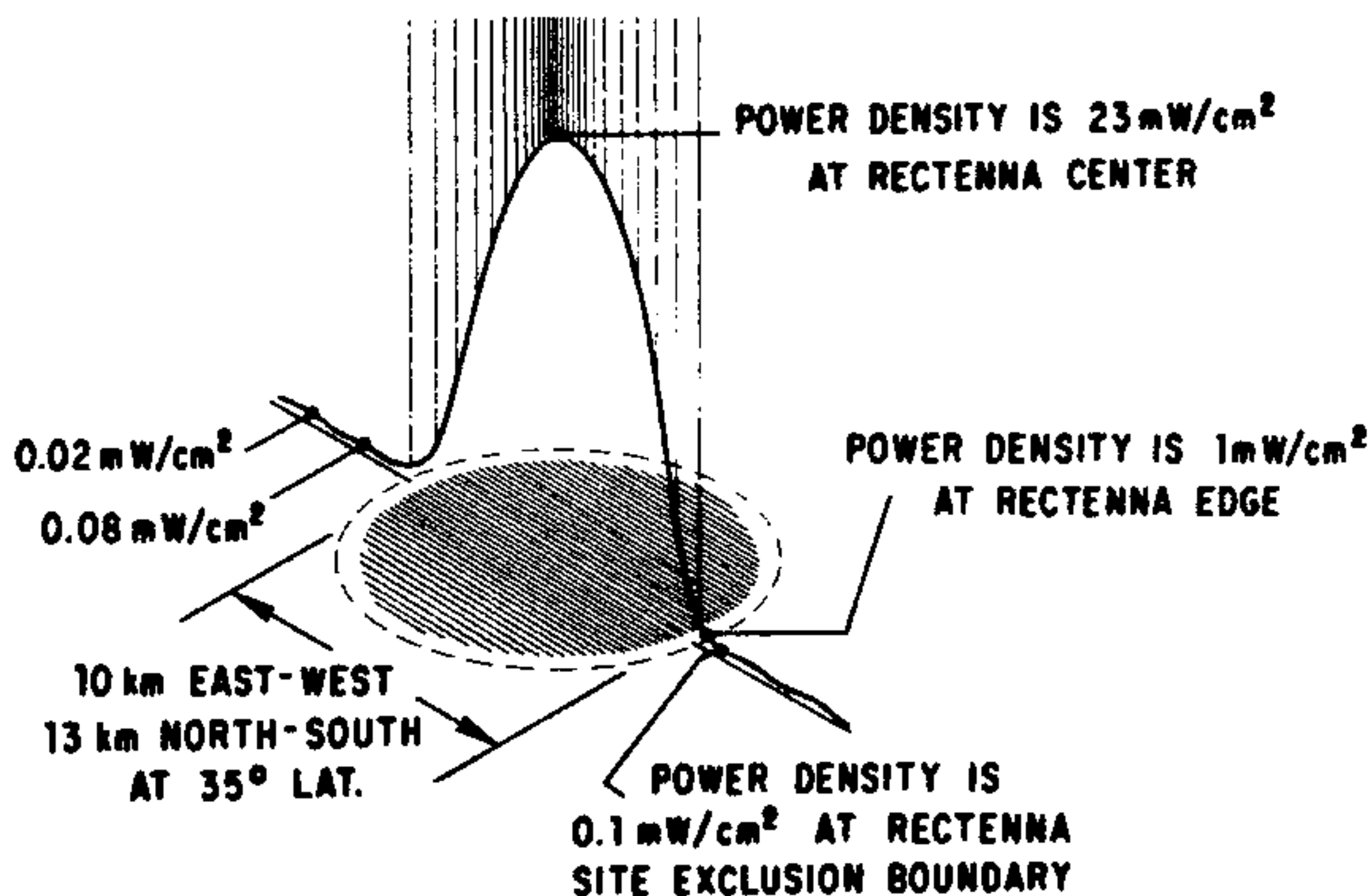
Fig. 1. SPS Microwave Power Density Characteristics at Rectenna Sites
