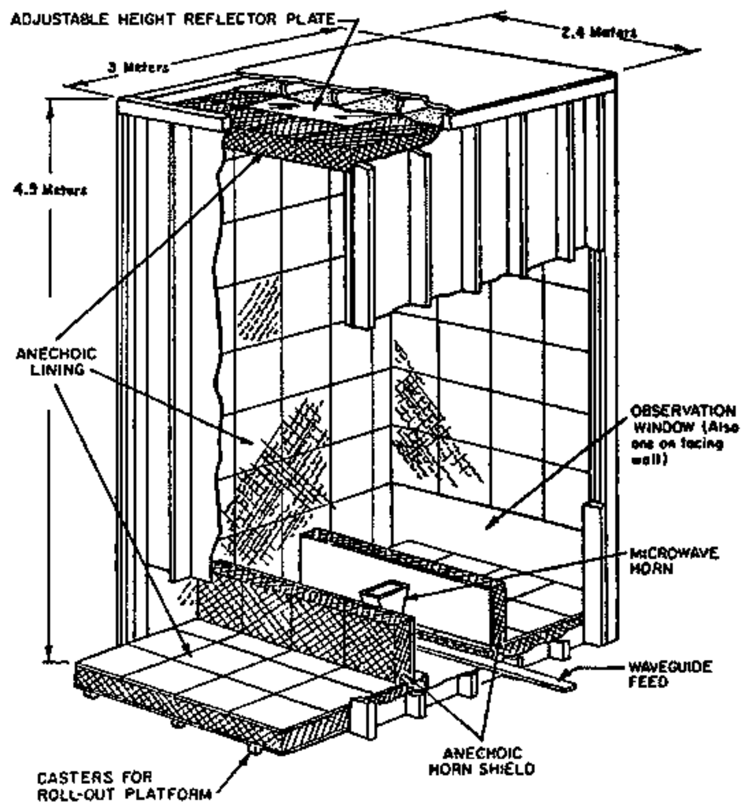
FIGURE 3. MICROWAVE IRRADIATION CHAMBER
