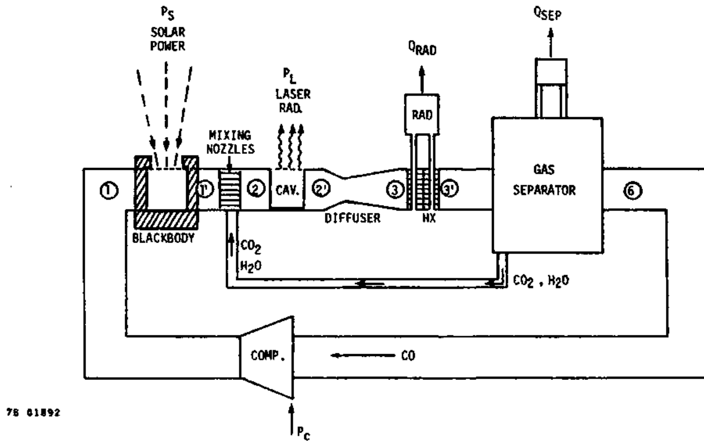
Figure 1. Indirect Optically Pumped CO/CO 2 Mixing Laser
