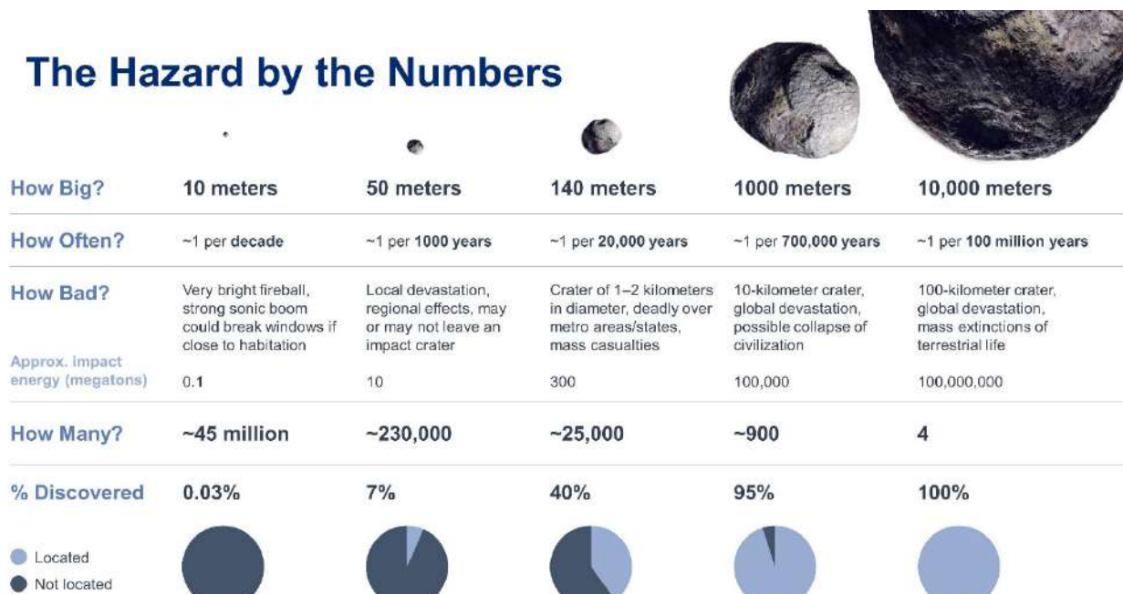
Figure 2: NEO size, frequency of Earth-impact, and hazard. (Credit: Johns Hopkins University/Applied Physics Laboratory)
