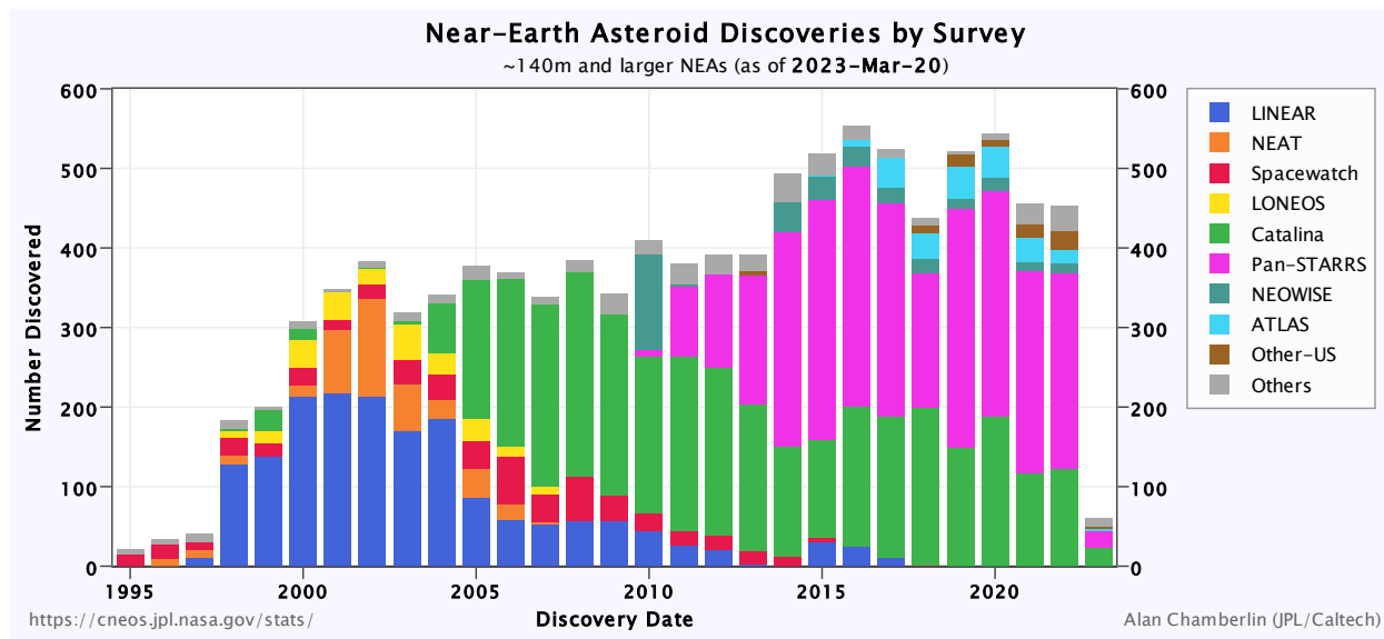
Figure 4: Large NEO Discoveries by Survey (Credit: NASA)
