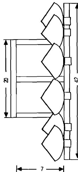
DIMENSIONS IN METERS
