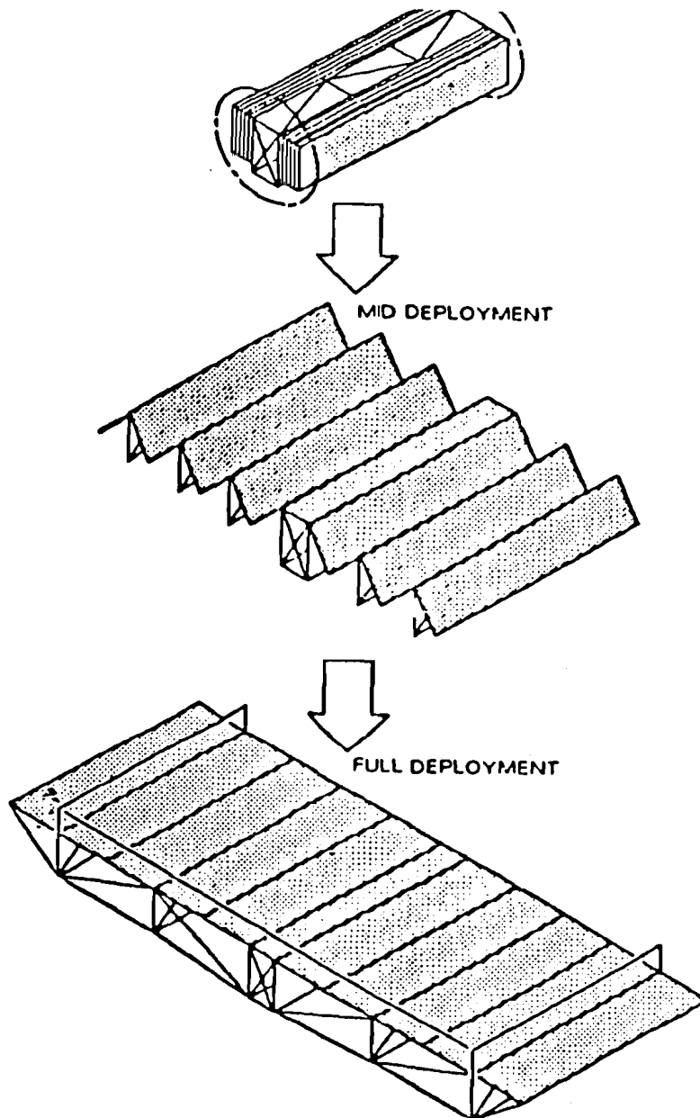
Figure 9. Deployment Sequence
