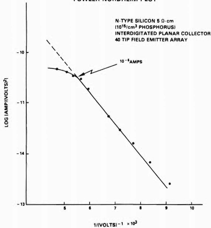
FOWLER-NORDHEIM PLOT
