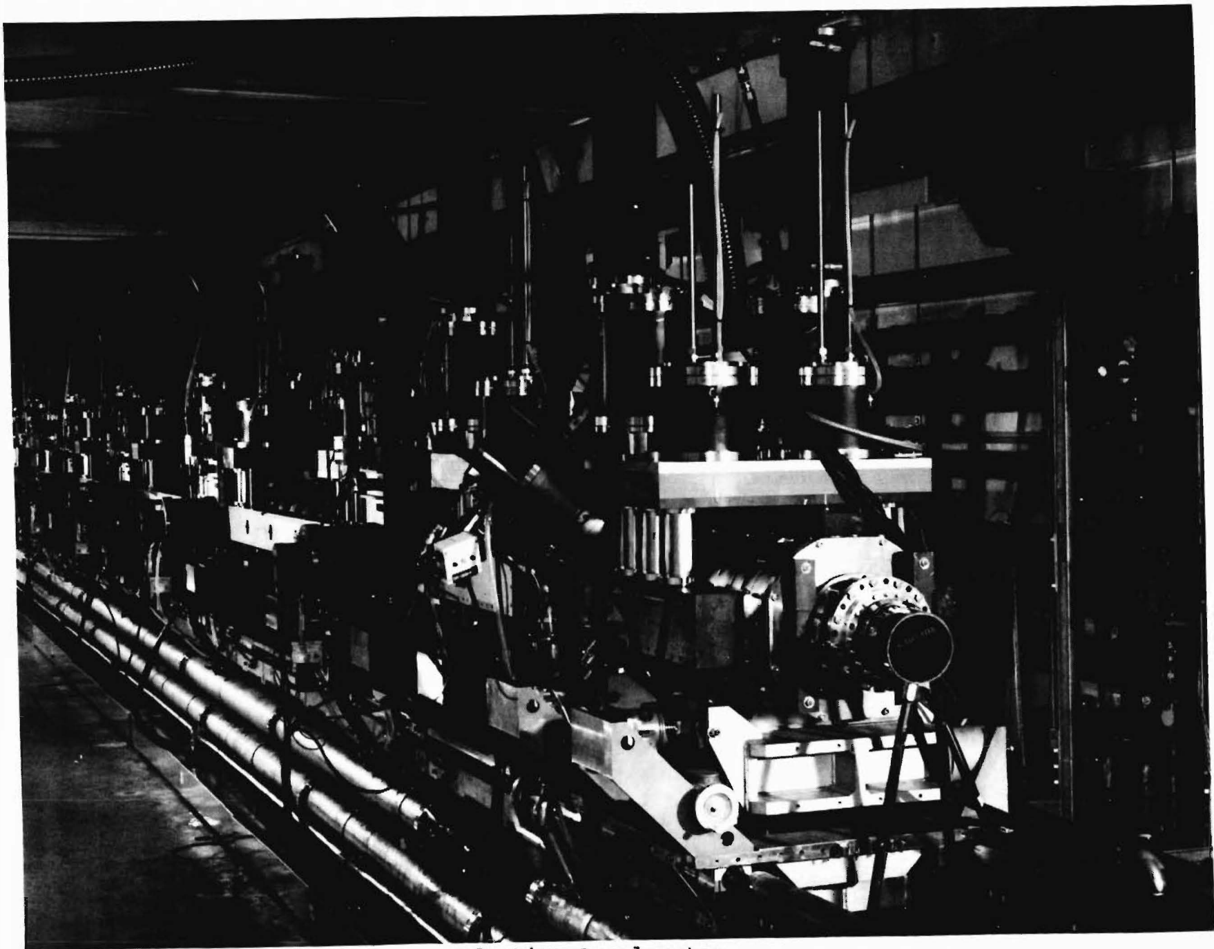
Induction Accelerator
