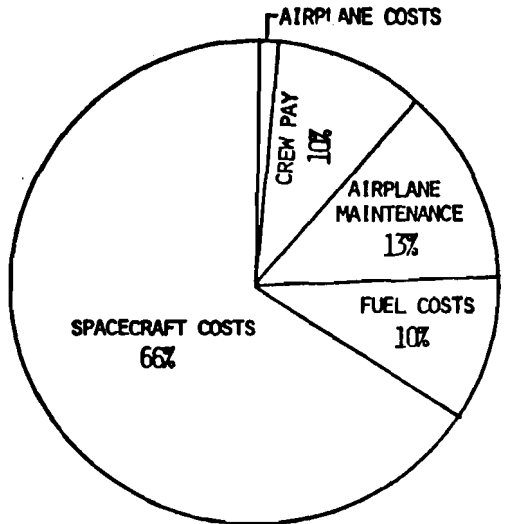
LASER FLIGHT SYSTEM COST $1.36/KG-PAYLOAD
