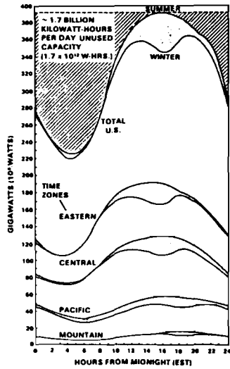
ESTIMATED TYPICAL DAILY ELECTRIC LOAD VARIATIONS FOR THE UNITED STATES IN 1985. STIPPLED AREAS INDICATE SEASONAL RANGE. LINED AREA REPRESENTS UNUSED OFF-LOAD CAPACITY.*
